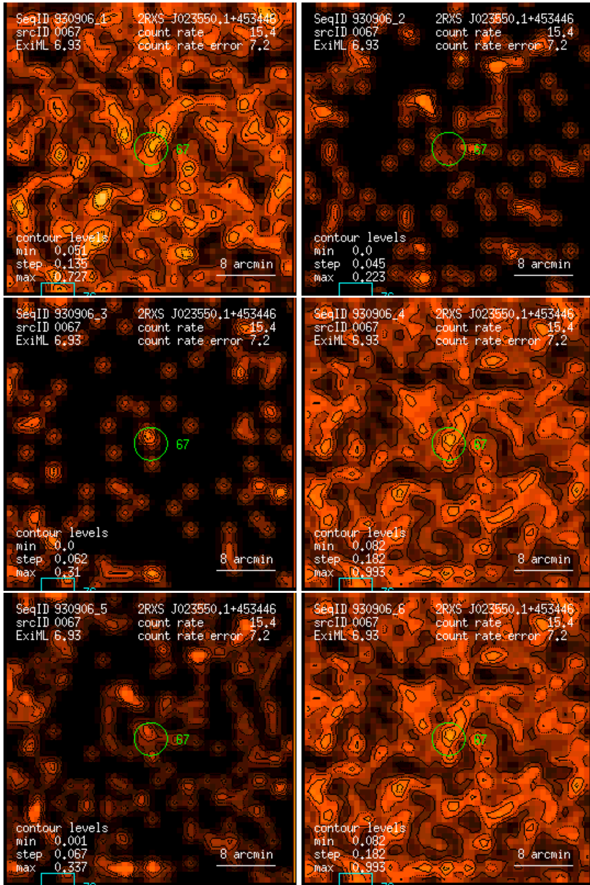
Figure 67: RASS 930906: detection 0067: band rate images, Gaussian filter: (1) PSPC channels 11 – 41, (2) 52 – 90, (3) 91 – 201, (4) 11 – 235, (5) 52 – 201, (6) 11 – 201. Broad band rates in counts/ks. Band rate contour levels in counts/ks/arcmin 2 .
