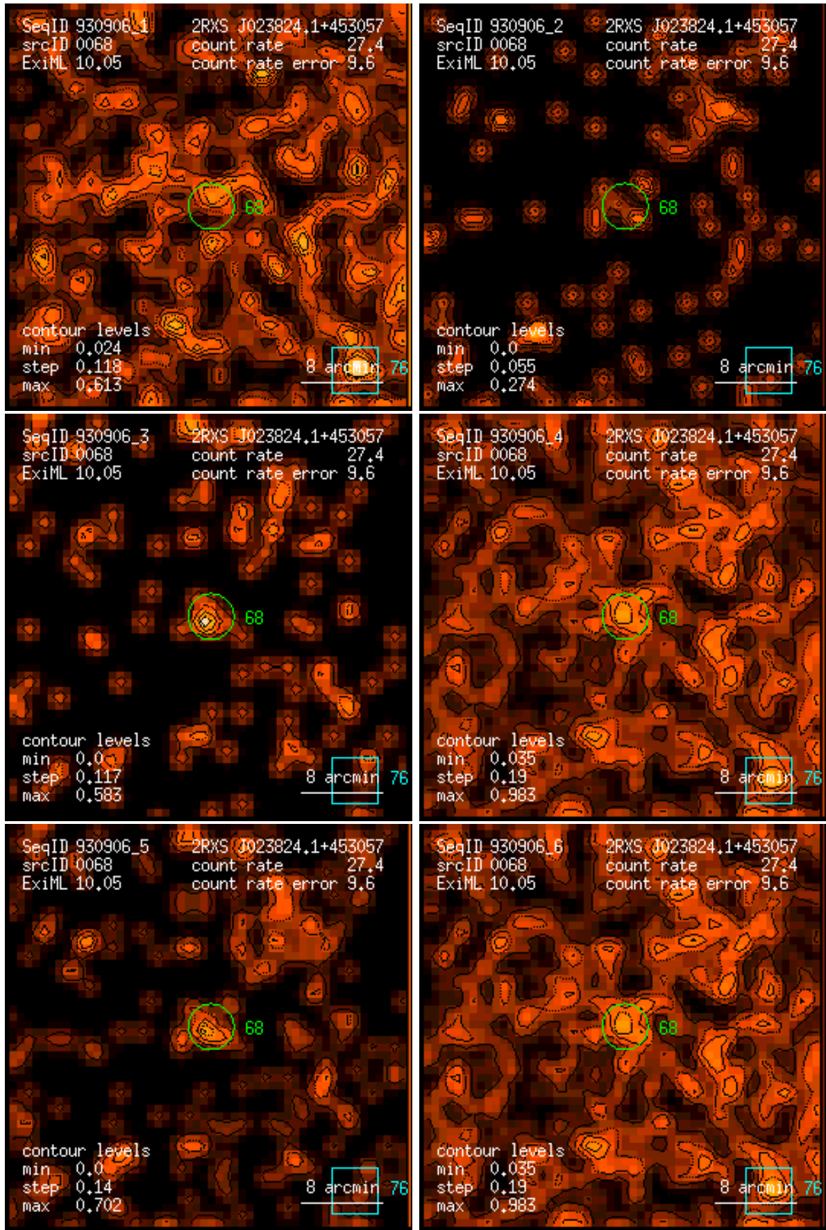
Figure 68: RASS 930906: detection 0068: band rate images, Gaussian filter: (1) PSPC channels 11 – 41, (2) 52 – 90, (3) 91 – 201, (4) 11 – 235, (5) 52 – 201, (6) 11 – 201. Broad band rates in counts/ks. Band rate contour levels in counts/ks/arcmin 2 .
