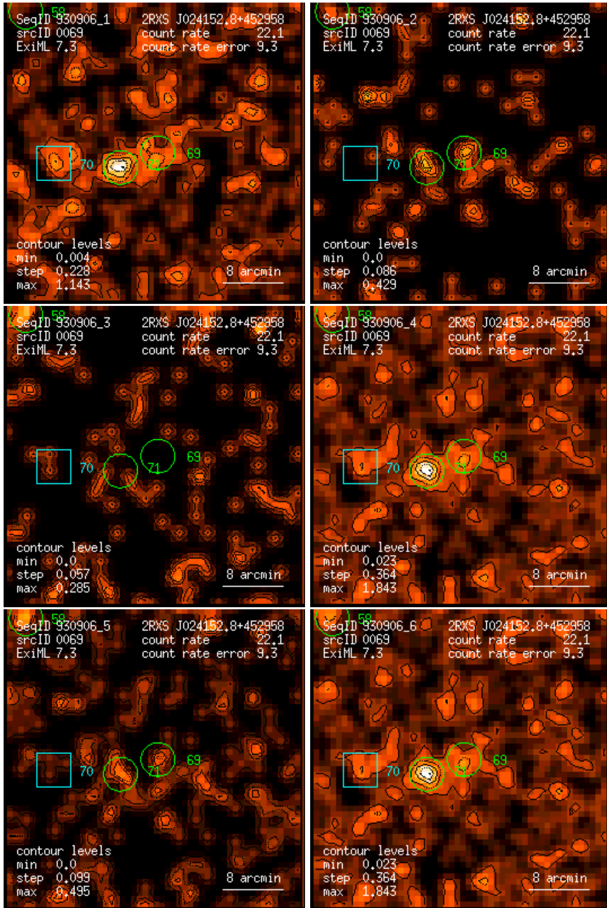
Figure 69: RASS 930906: detection 0069: band rate images, Gaussian filter: (1) PSPC channels 11 – 41, (2) 52 – 90, (3) 91 – 201, (4) 11 – 235, (5) 52 – 201, (6) 11 – 201. Broad band rates in counts/ks. Band rate contour levels in counts/ks/arcmin 2 .
