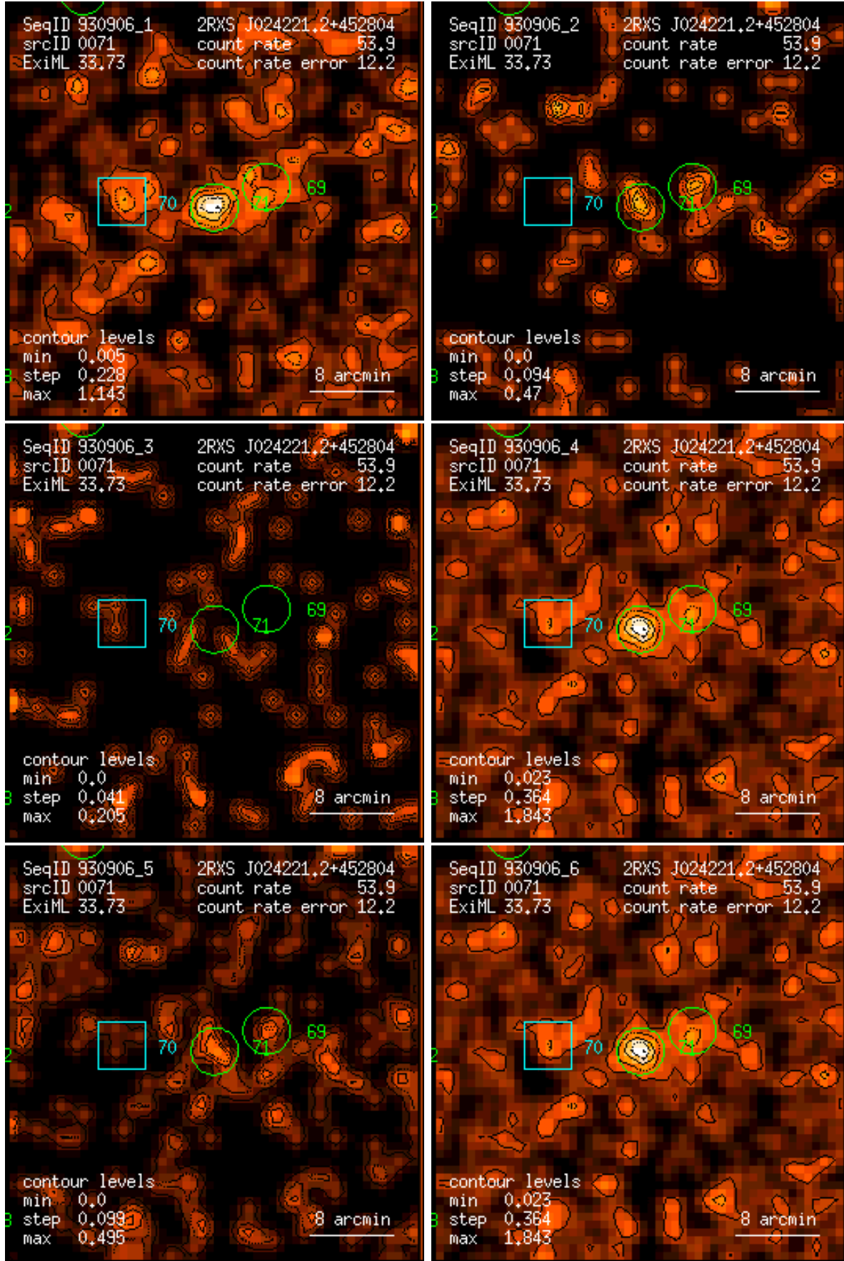
Figure 71: RASS 930906: detection 0071: band rate images, Gaussian filter: (1) PSPC channels 11 – 41, (2) 52 – 90, (3) 91 – 201, (4) 11 – 235, (5) 52 – 201, (6) 11 – 201. Broad band rates in counts/ks. Band rate contour levels in counts/ks/arcmin 2 .
