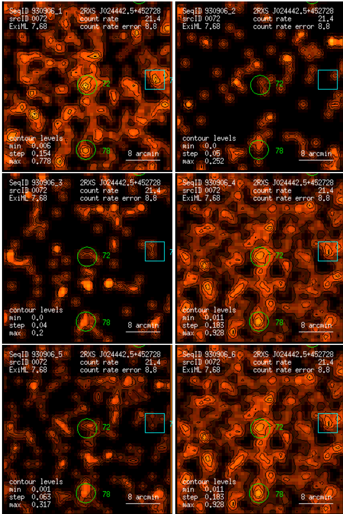
Figure 72: RASS 930906: detection 0072: band rate images, Gaussian filter: (1) PSPC channels 11 – 41, (2) 52 – 90, (3) 91 – 201, (4) 11 – 235, (5) 52 – 201, (6) 11 – 201. Broad band rates in counts/ks. Band rate contour levels in counts/ks/arcmin 2 .
