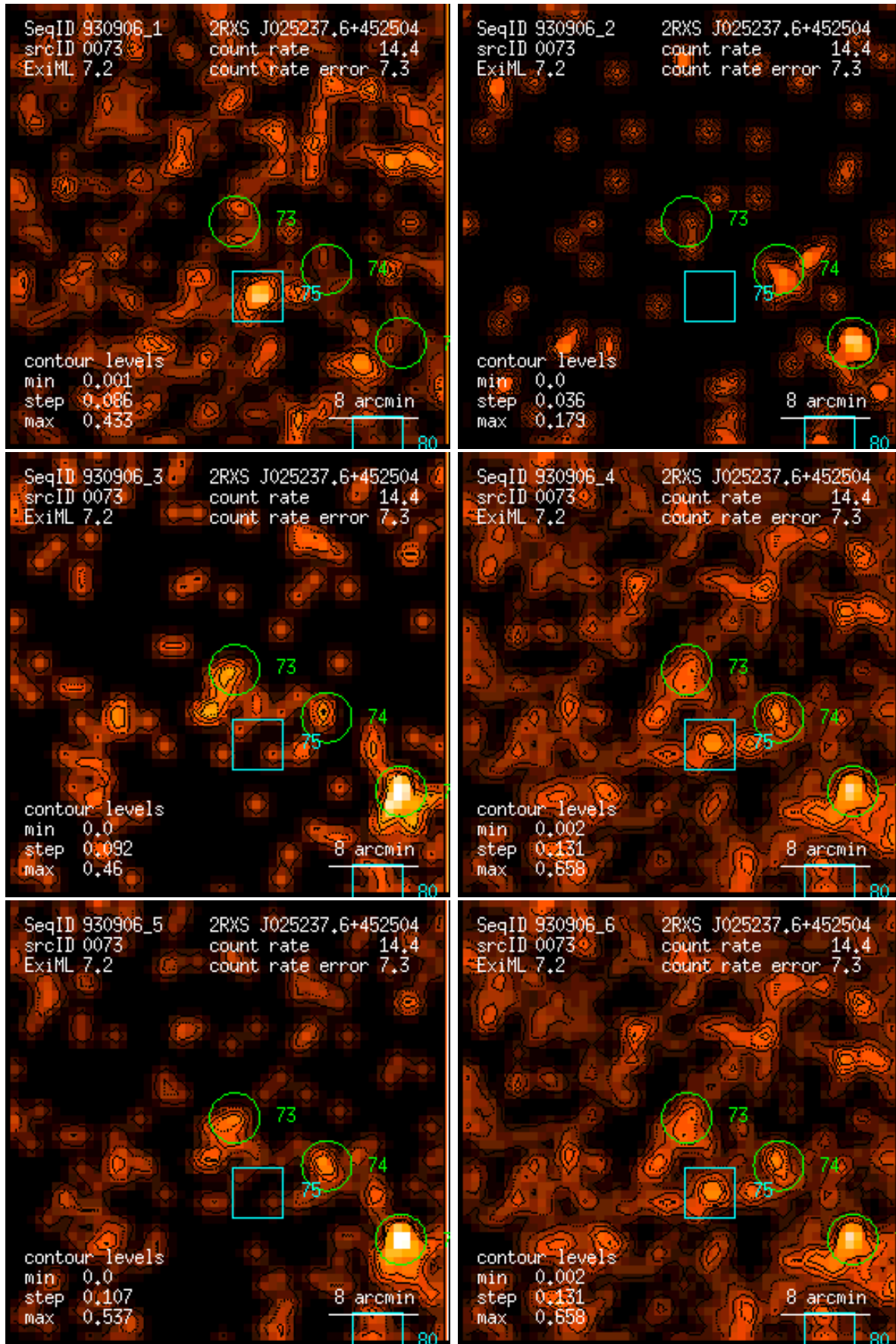
Figure 73: RASS 930906: detection 0073: band rate images, Gaussian filter: (1) PSPC channels 11 – 41, (2) 52 – 90, (3) 91 – 201, (4) 11 – 235, (5) 52 – 201, (6) 11 – 201. Broad band rates in counts/ks. Band rate contour levels in counts/ks/arcmin 2 .
