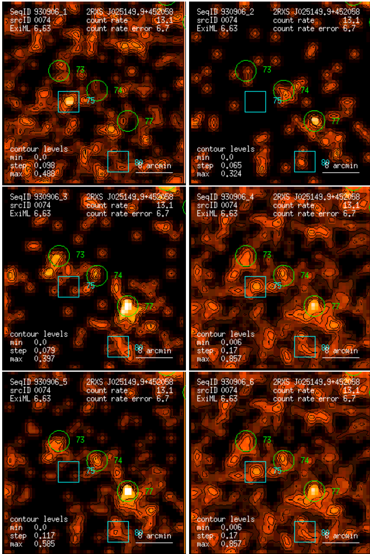
Figure 74: RASS 930906: detection 0074: band rate images, Gaussian filter: (1) PSPC channels 11 – 41, (2) 52 – 90, (3) 91 – 201, (4) 11 – 235, (5) 52 – 201, (6) 11 – 201. Broad band rates in counts/ks. Band rate contour levels in counts/ks/arcmin 2 .
