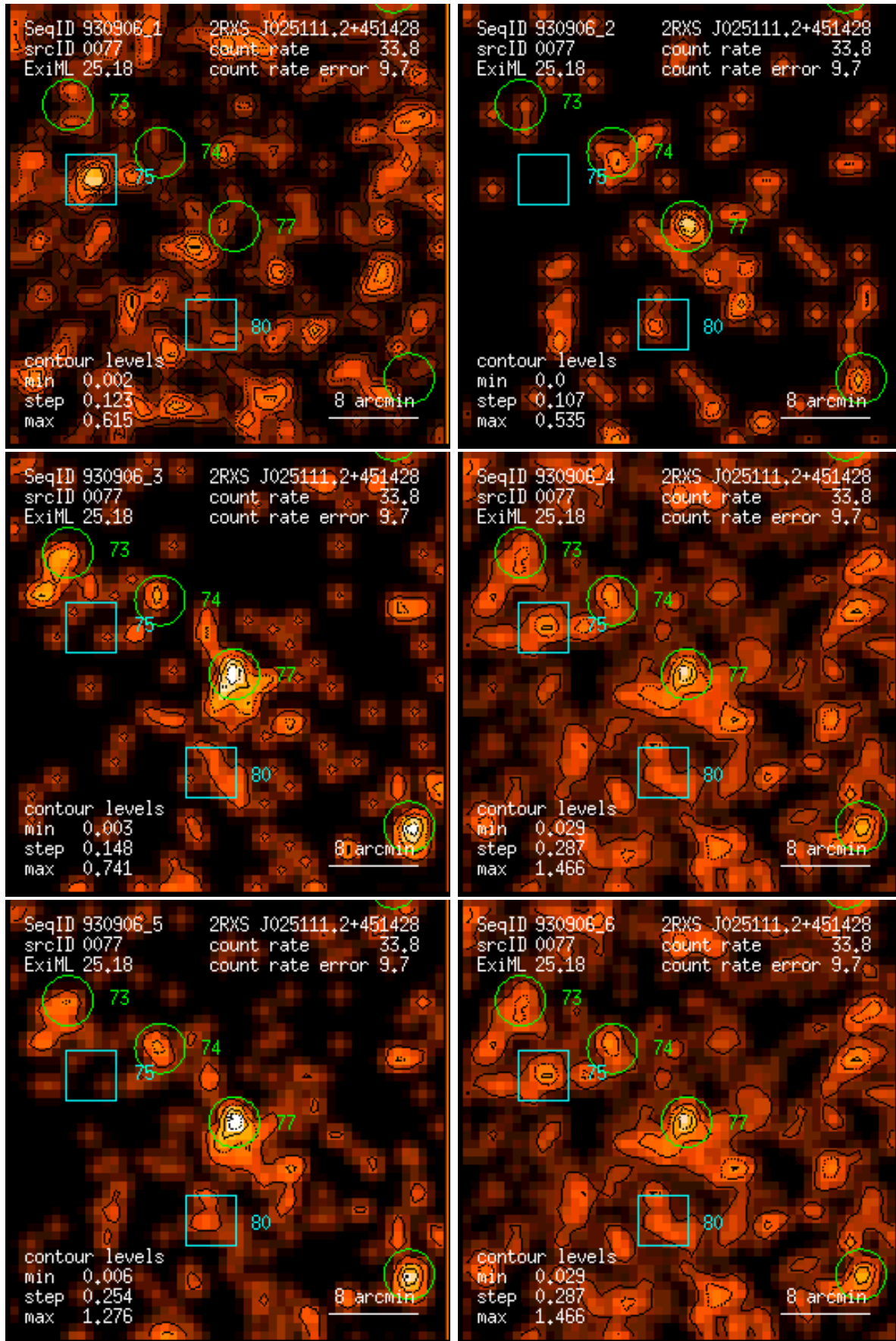
Figure 77: RASS 930906: detection 0077: band rate images, Gaussian filter: (1) PSPC channels 11 – 41, (2) 52 – 90, (3) 91 – 201, (4) 11 – 235, (5) 52 – 201, (6) 11 – 201. Broad band rates in counts/ks. Band rate contour levels in counts/ks/arcmin 2 .
