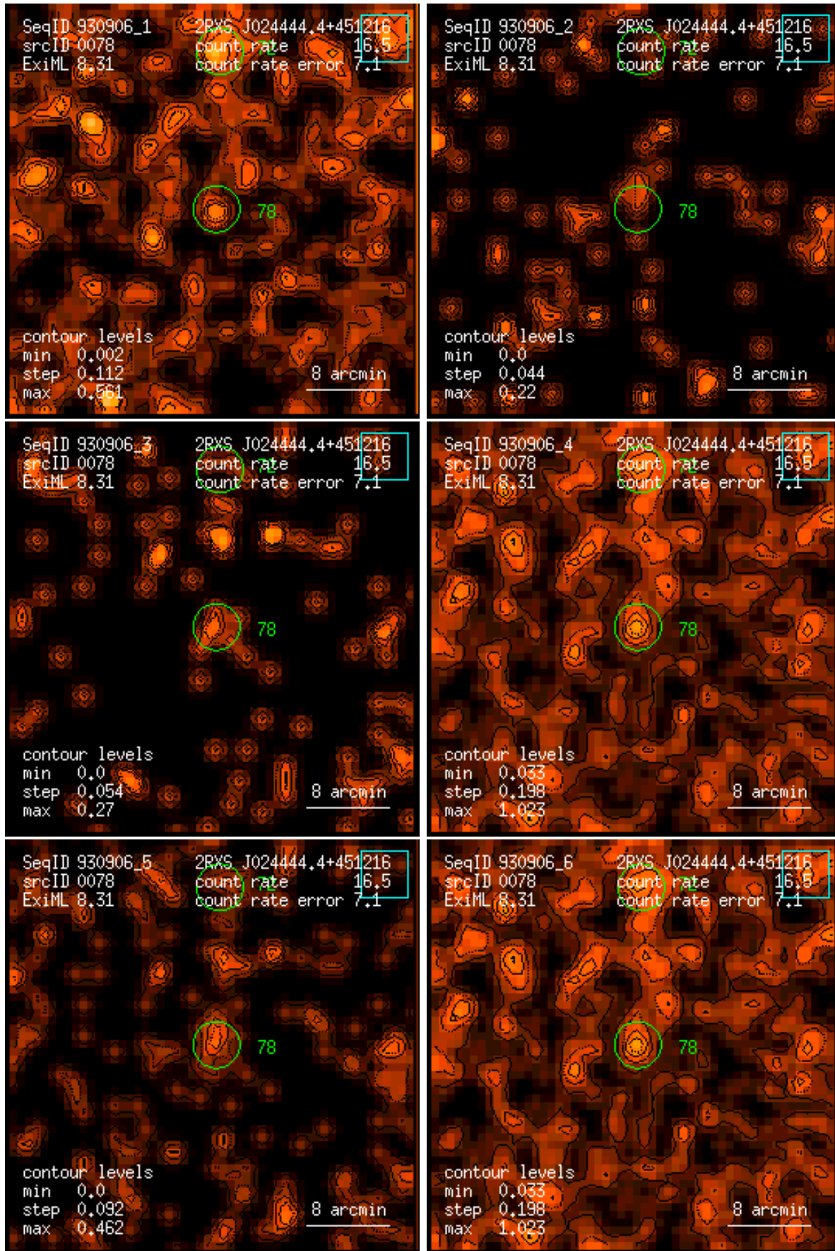
Figure 78: RASS 930906: detection 0078: band rate images, Gaussian filter: (1) PSPC channels 11 – 41, (2) 52 – 90, (3) 91 – 201, (4) 11 – 235, (5) 52 – 201, (6) 11 – 201. Broad band rates in counts/ks. Band rate contour levels in counts/ks/arcmin 2 .
