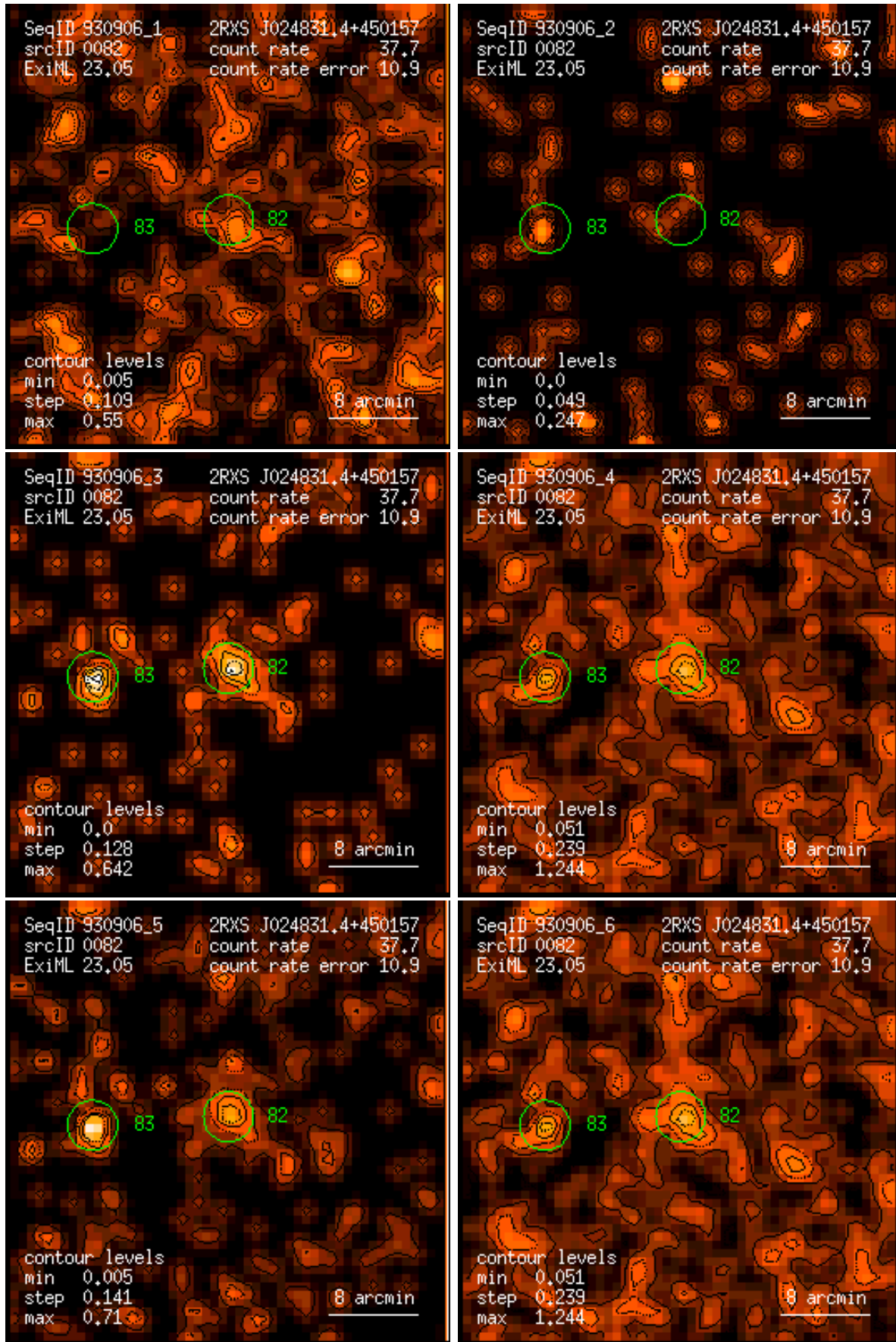
Figure 82: RASS 930906: detection 0082: band rate images, Gaussian filter: (1) PSPC channels 11 – 41, (2) 52 – 90, (3) 91 – 201, (4) 11 – 235, (5) 52 – 201, (6) 11 – 201. Broad band rates in counts/ks. Band rate contour levels in counts/ks/arcmin 2 .
