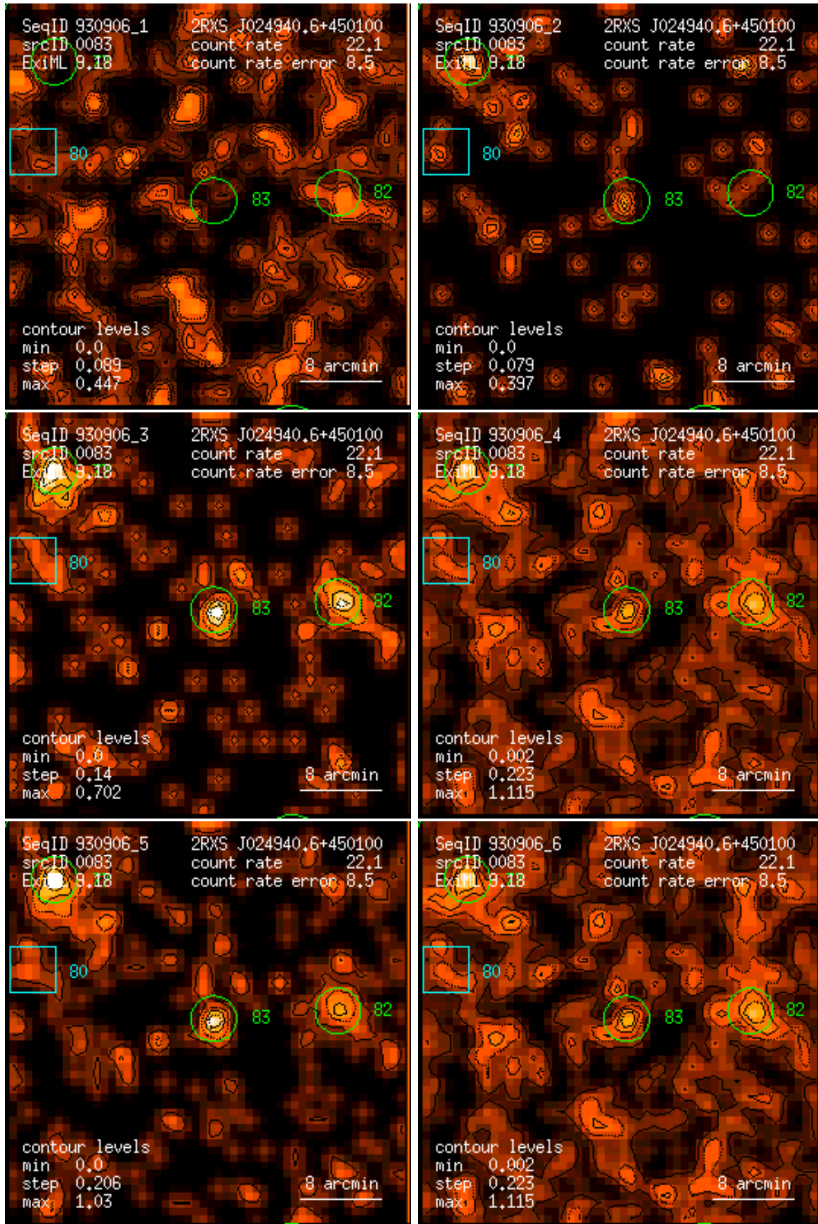
Figure 83: RASS 930906: detection 0083: band rate images, Gaussian filter: (1) PSPC channels 11 – 41, (2) 52 – 90, (3) 91 – 201, (4) 11 – 235, (5) 52 – 201, (6) 11 – 201. Broad band rates in counts/ks. Band rate contour levels in counts/ks/arcmin 2 .
