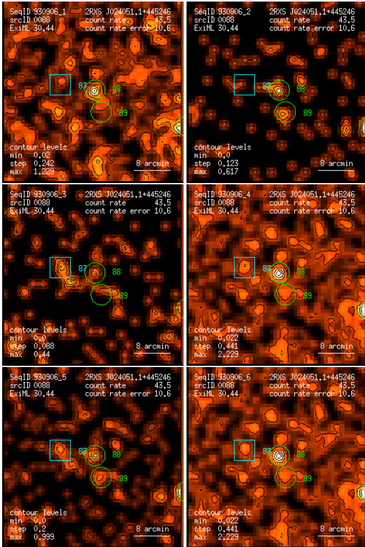
Figure 88: RASS 930906: detection 0088: band rate images, Gaussian filter: (1) PSPC channels 11 – 41, (2) 52 – 90, (3) 91 – 201, (4) 11 – 235, (5) 52 – 201, (6) 11 – 201. Broad band rates in counts/ks. Band rate contour levels in counts/ks/arcmin 2 .
