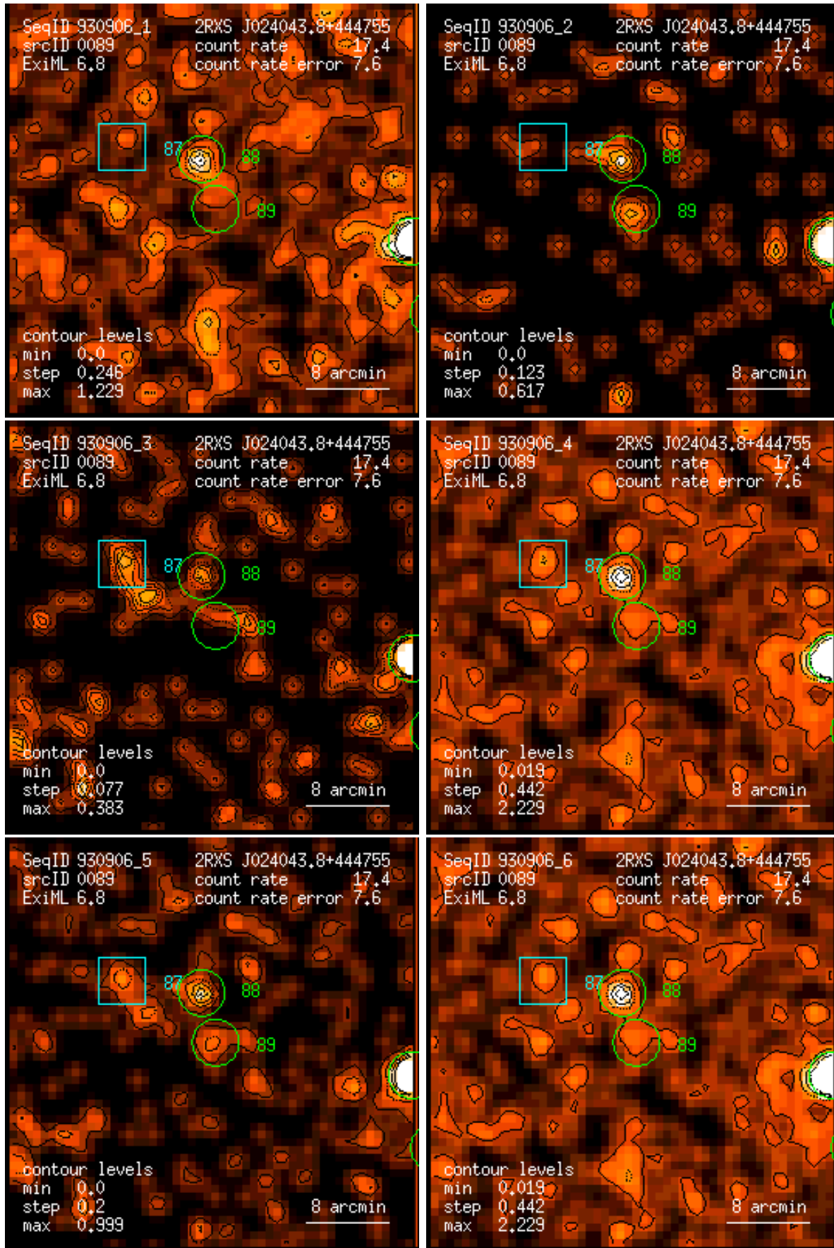
Figure 89: RASS 930906: detection 0089: band rate images, Gaussian filter: (1) PSPC channels 11 – 41, (2) 52 – 90, (3) 91 – 201, (4) 11 – 235, (5) 52 – 201, (6) 11 – 201. Broad band rates in counts/ks. Band rate contour levels in counts/ks/arcmin 2 .
