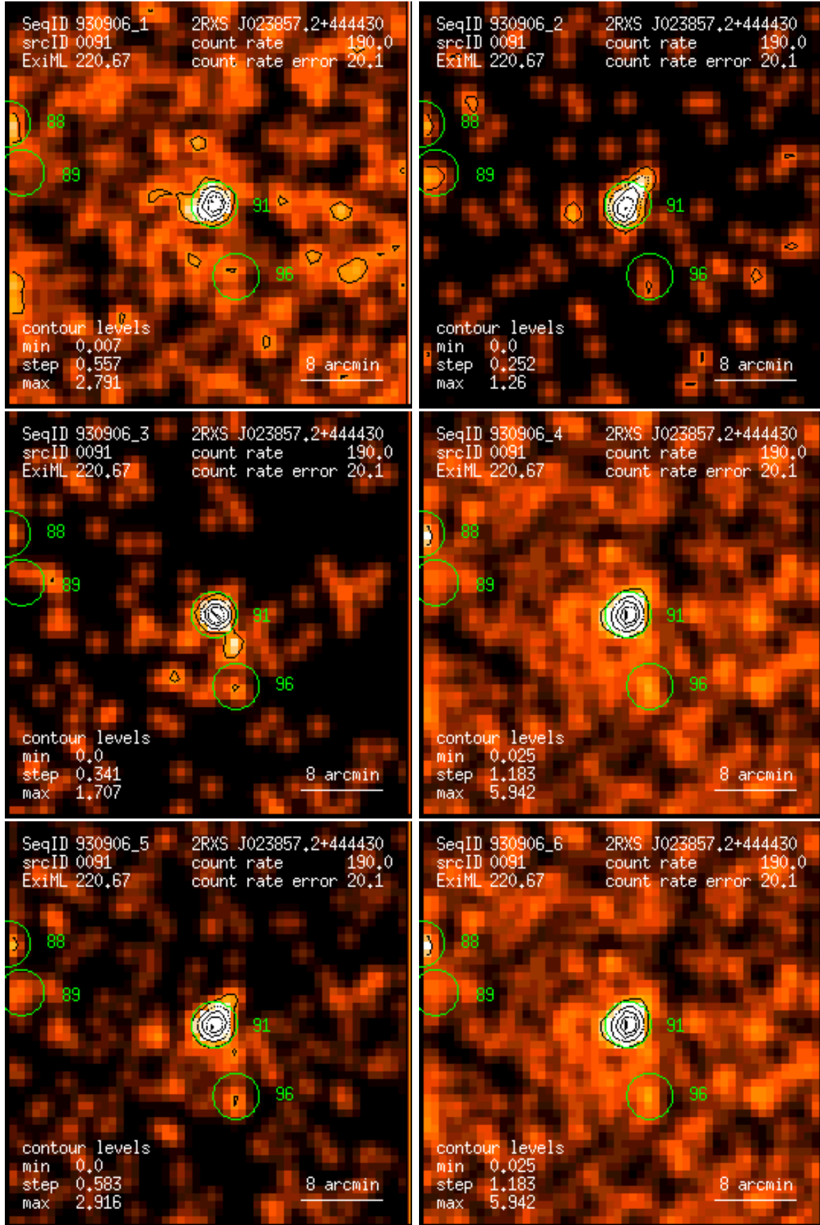
Figure 91: RASS 930906: detection 0091: band rate images, Gaussian filter: (1) PSPC channels 11 – 41, (2) 52 – 90, (3) 91 – 201, (4) 11 – 235, (5) 52 – 201, (6) 11 – 201. Broad band rates in counts/ks. Band rate contour levels in counts/ks/arcmin 2 .
