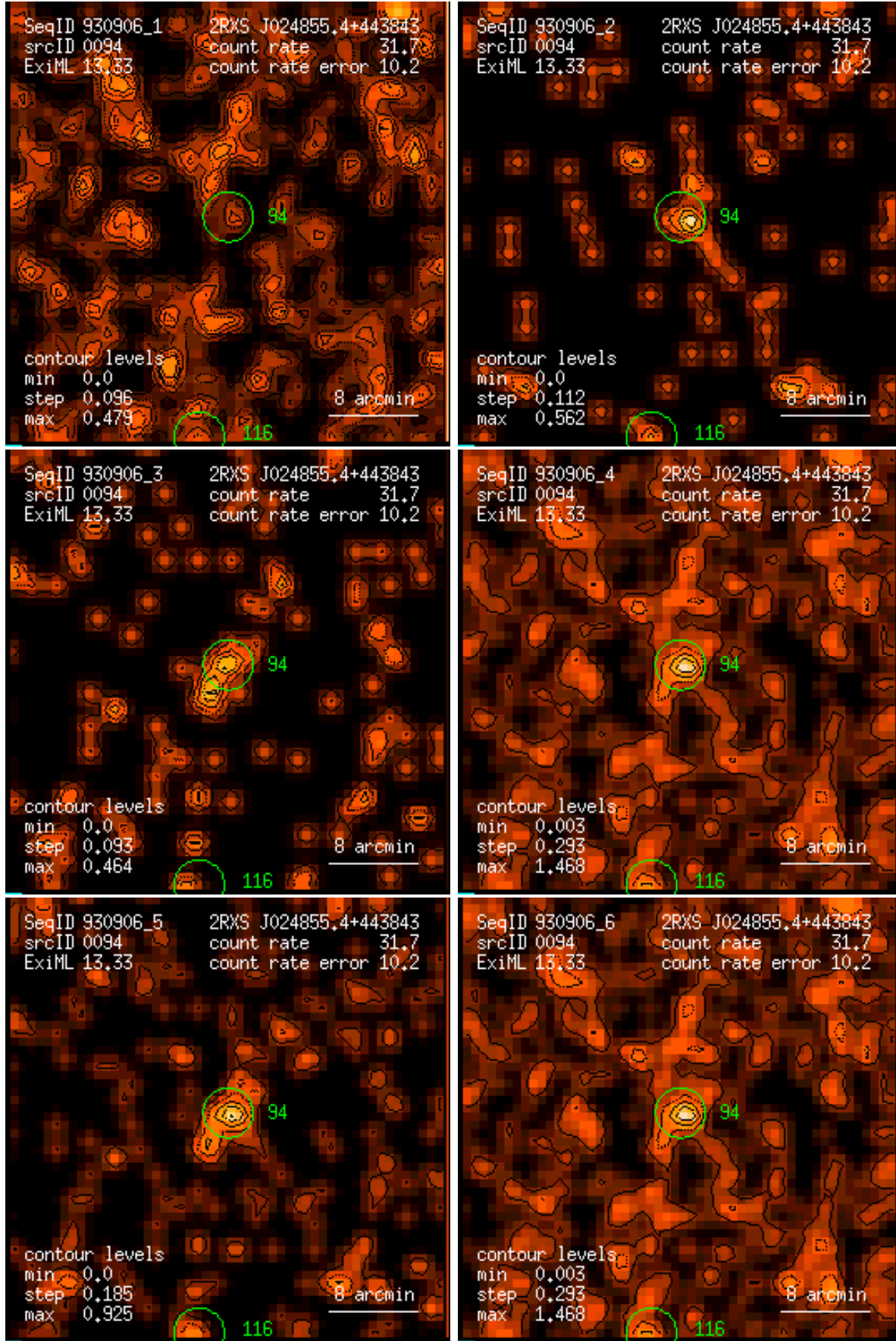
Figure 94: RASS 930906: detection 0094: band rate images, Gaussian filter: (1) PSPC channels 11 – 41, (2) 52 – 90, (3) 91 – 201, (4) 11 – 235, (5) 52 – 201, (6) 11 – 201. Broad band rates in counts/ks. Band rate contour levels in counts/ks/arcmin 2 .
