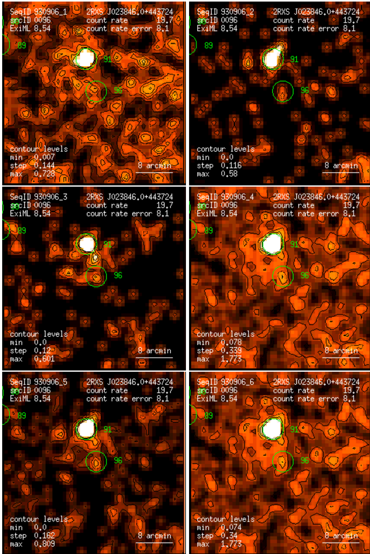
Figure 96: RASS 930906: detection 0096: band rate images, Gaussian filter: (1) PSPC channels 11 – 41, (2) 52 – 90, (3) 91 – 201, (4) 11 – 235, (5) 52 – 201, (6) 11 – 201. Broad band rates in counts/ks. Band rate contour levels in counts/ks/arcmin 2 .
