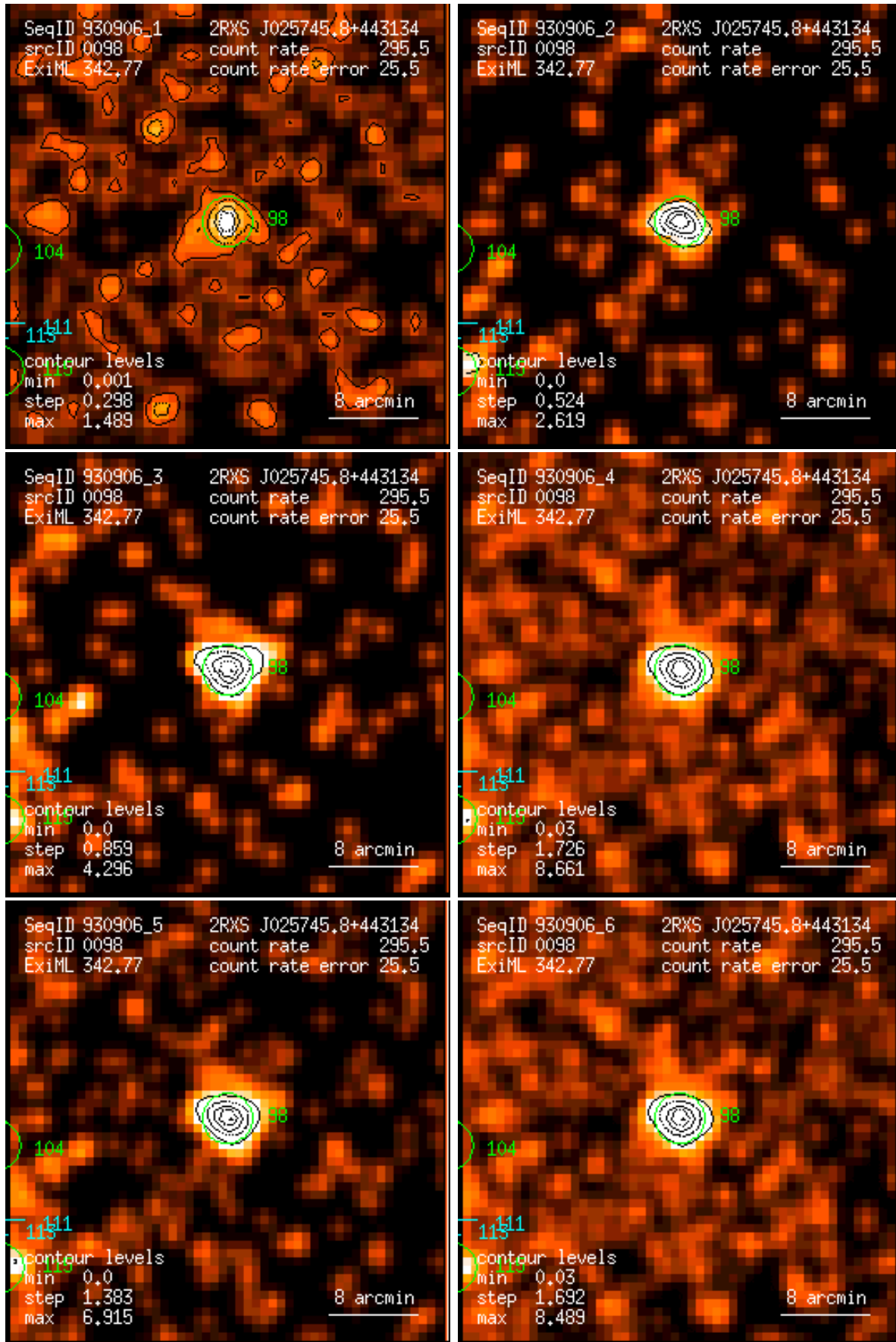
Figure 98: RASS 930906: detection 0098: band rate images, Gaussian filter: (1) PSPC channels 11 – 41, (2) 52 – 90, (3) 91 – 201, (4) 11 – 235, (5) 52 – 201, (6) 11 – 201. Broad band rates in counts/ks. Band rate contour levels in counts/ks/arcmin 2 .
