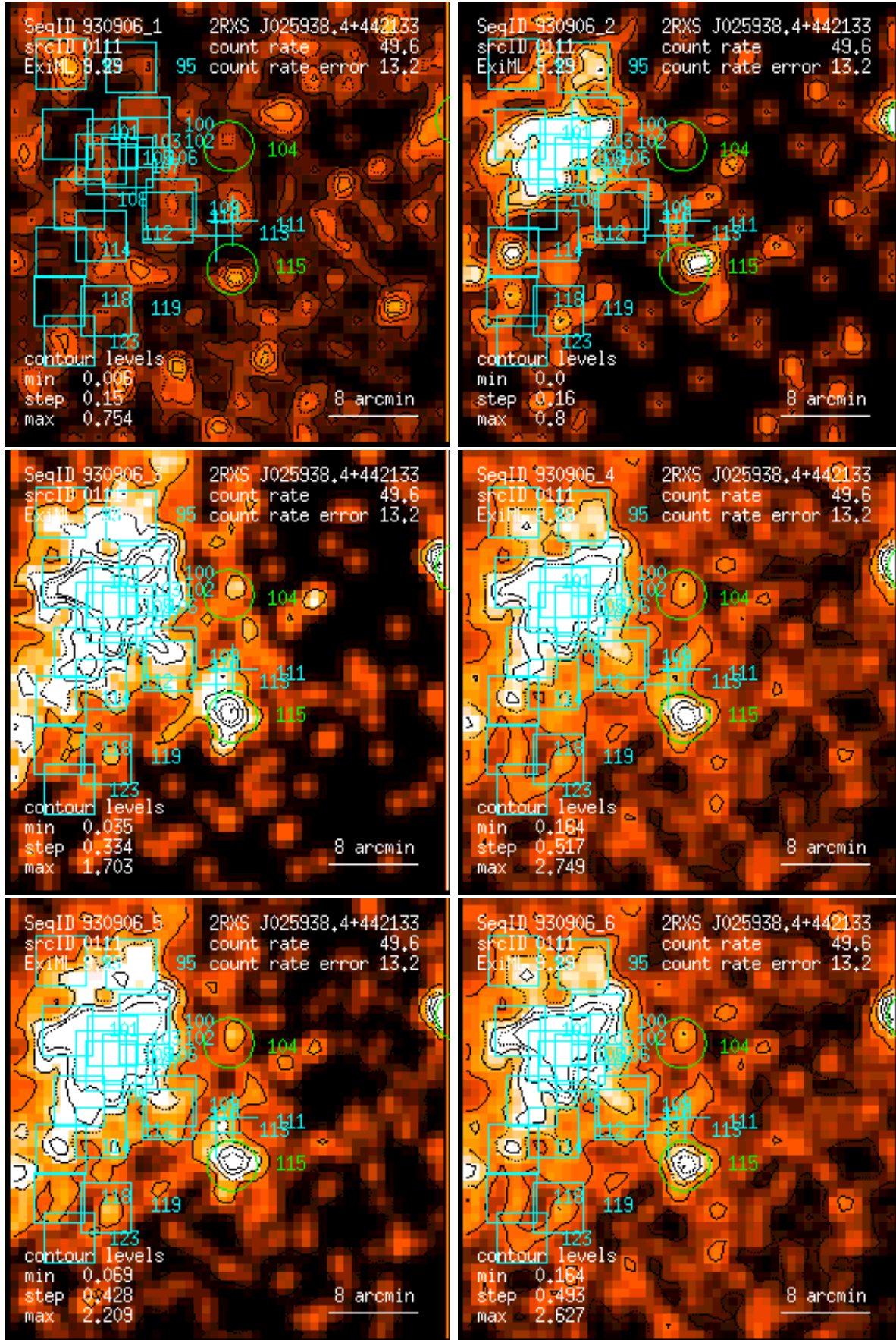
Figure 111: RASS 930906: detection 0111: band rate images, Gaussian filter: (1) PSPC channels 11 – 41, (2) 52 – 90, (3) 91 – 201, (4) 11 – 235, (5) 52 – 201, (6) 11 – 201. Broad band rates in counts/ks. Band rate contour levels in counts/ks/arcmin 2 .
