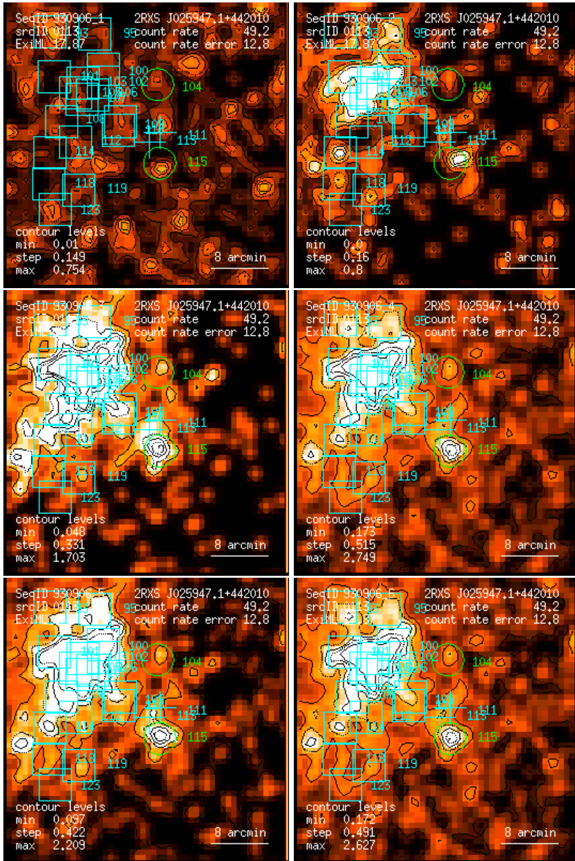
Figure 113: RASS 930906: detection 0113: band rate images, Gaussian filter: (1) PSPC channels 11 – 41, (2) 52 – 90, (3) 91 – 201, (4) 11 – 235, (5) 52 – 201, (6) 11 – 201. Broad band rates in counts/ks. Band rate contour levels in counts/ks/arcmin 2 .
