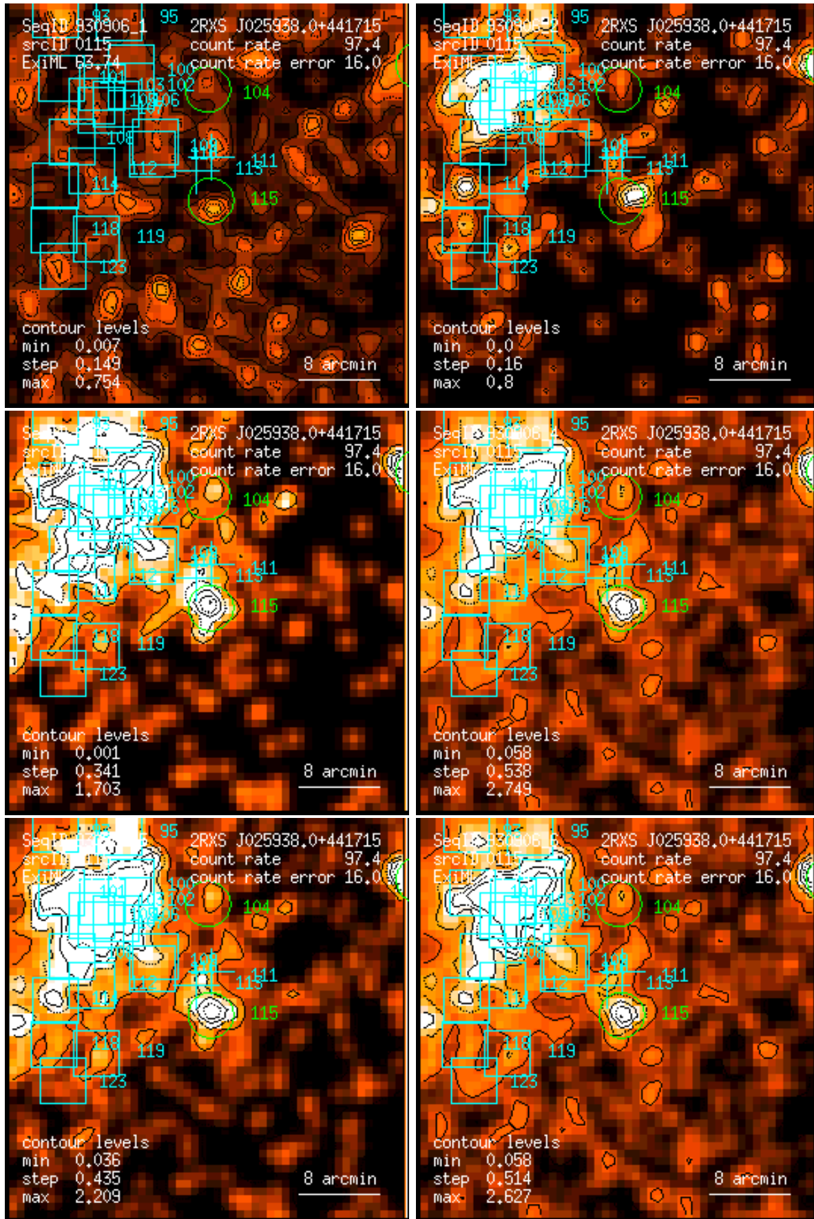
Figure 115: RASS 930906: detection 0115: band rate images, Gaussian filter: (1) PSPC channels 11 – 41, (2) 52 – 90, (3) 91 – 201, (4) 11 – 235, (5) 52 – 201, (6) 11 – 201. Broad band rates in counts/ks. Band rate contour levels in counts/ks/arcmin 2 .
