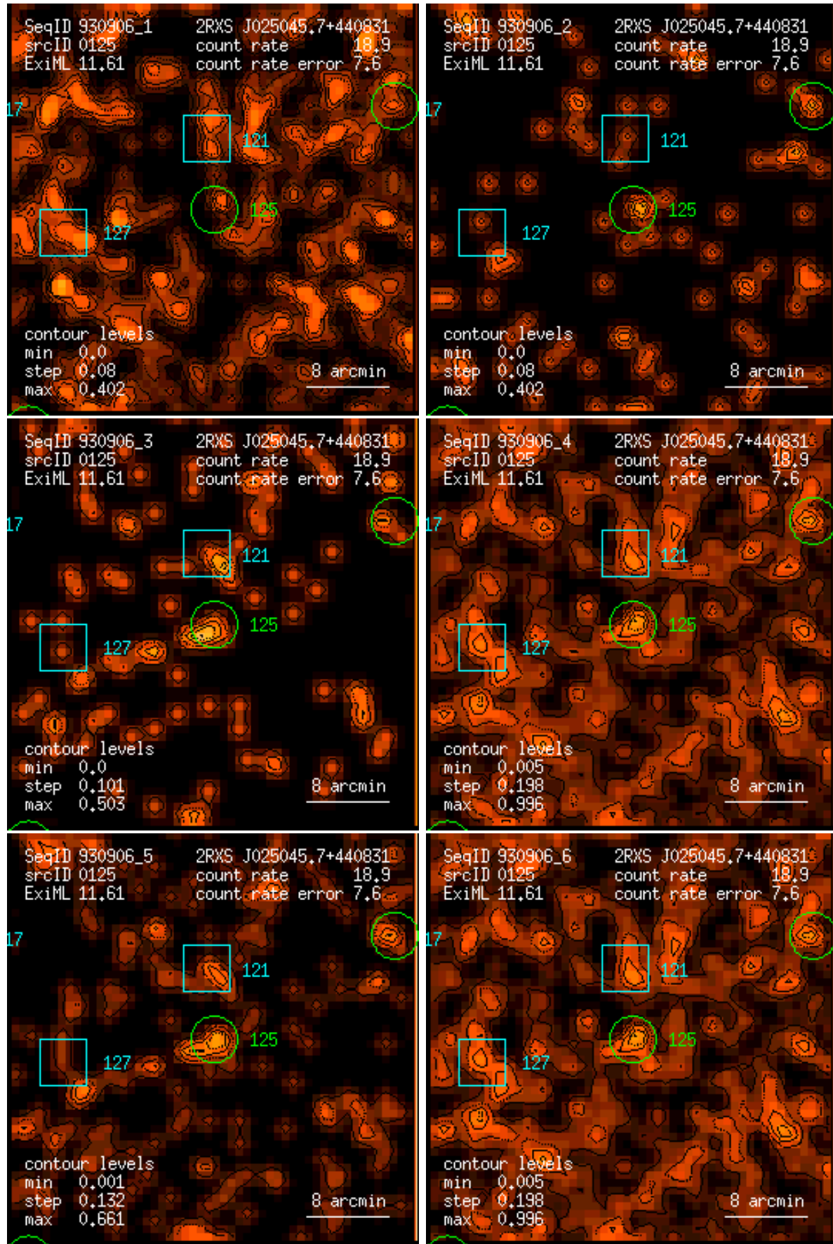
Figure 125: RASS 930906: detection 0125: band rate images, Gaussian filter: (1) PSPC channels 11 – 41, (2) 52 – 90, (3) 91 – 201, (4) 11 – 235, (5) 52 – 201, (6) 11 – 201. Broad band rates in counts/ks. Band rate contour levels in counts/ks/arcmin 2 .
