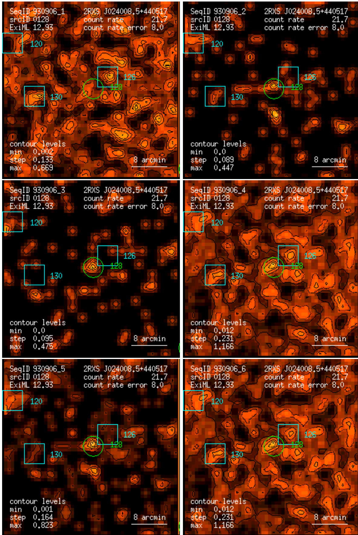
Figure 128: RASS 930906: detection 0128: band rate images, Gaussian filter: (1) PSPC channels 11 – 41, (2) 52 – 90, (3) 91 – 201, (4) 11 – 235, (5) 52 – 201, (6) 11 – 201. Broad band rates in counts/ks. Band rate contour levels in counts/ks/arcmin 2 .
