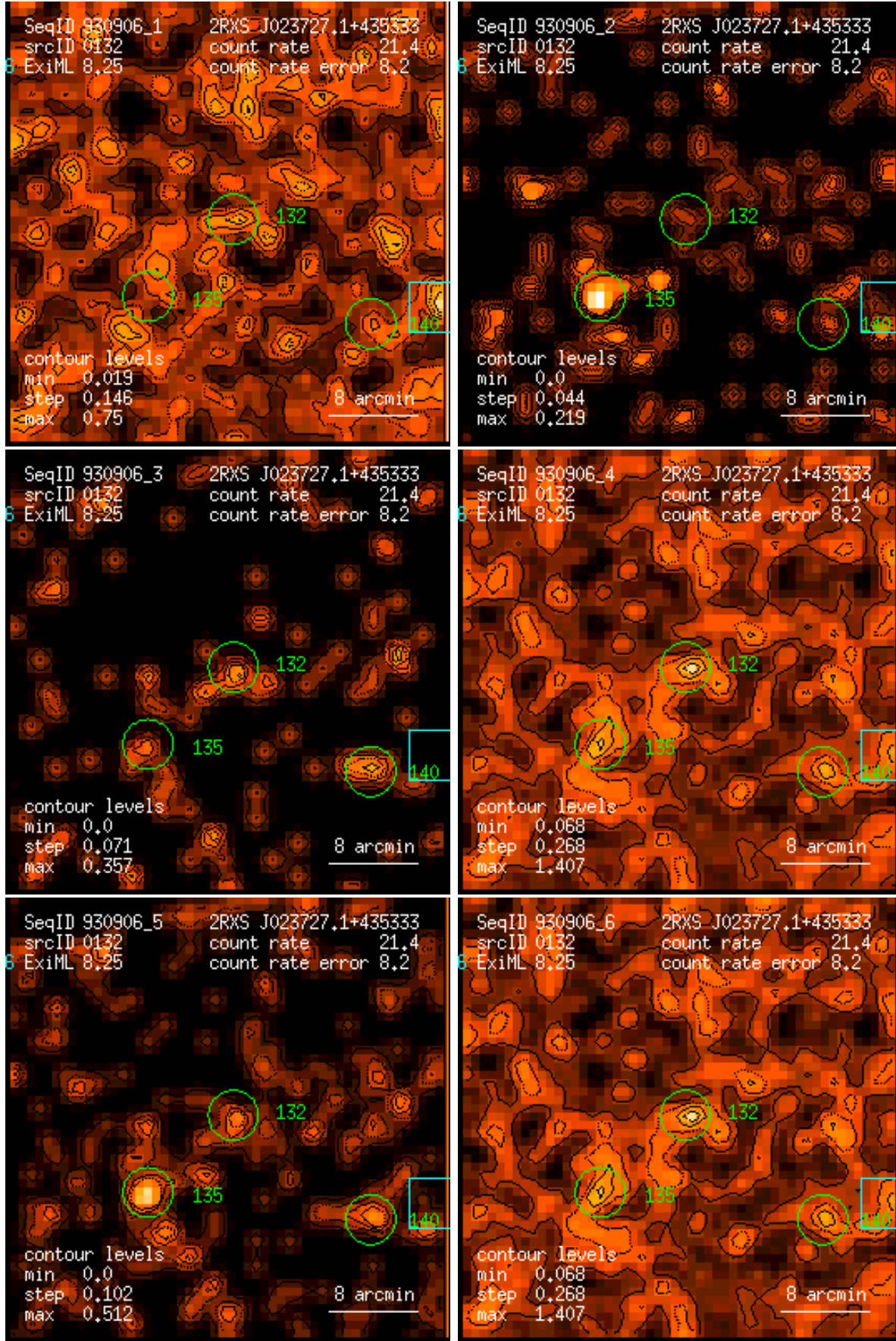
Figure 132: RASS 930906: detection 0132: band rate images, Gaussian filter: (1) PSPC channels 11 – 41, (2) 52 – 90, (3) 91 – 201, (4) 11 – 235, (5) 52 – 201, (6) 11 – 201. Broad band rates in counts/ks. Band rate contour levels in counts/ks/arcmin 2 .
