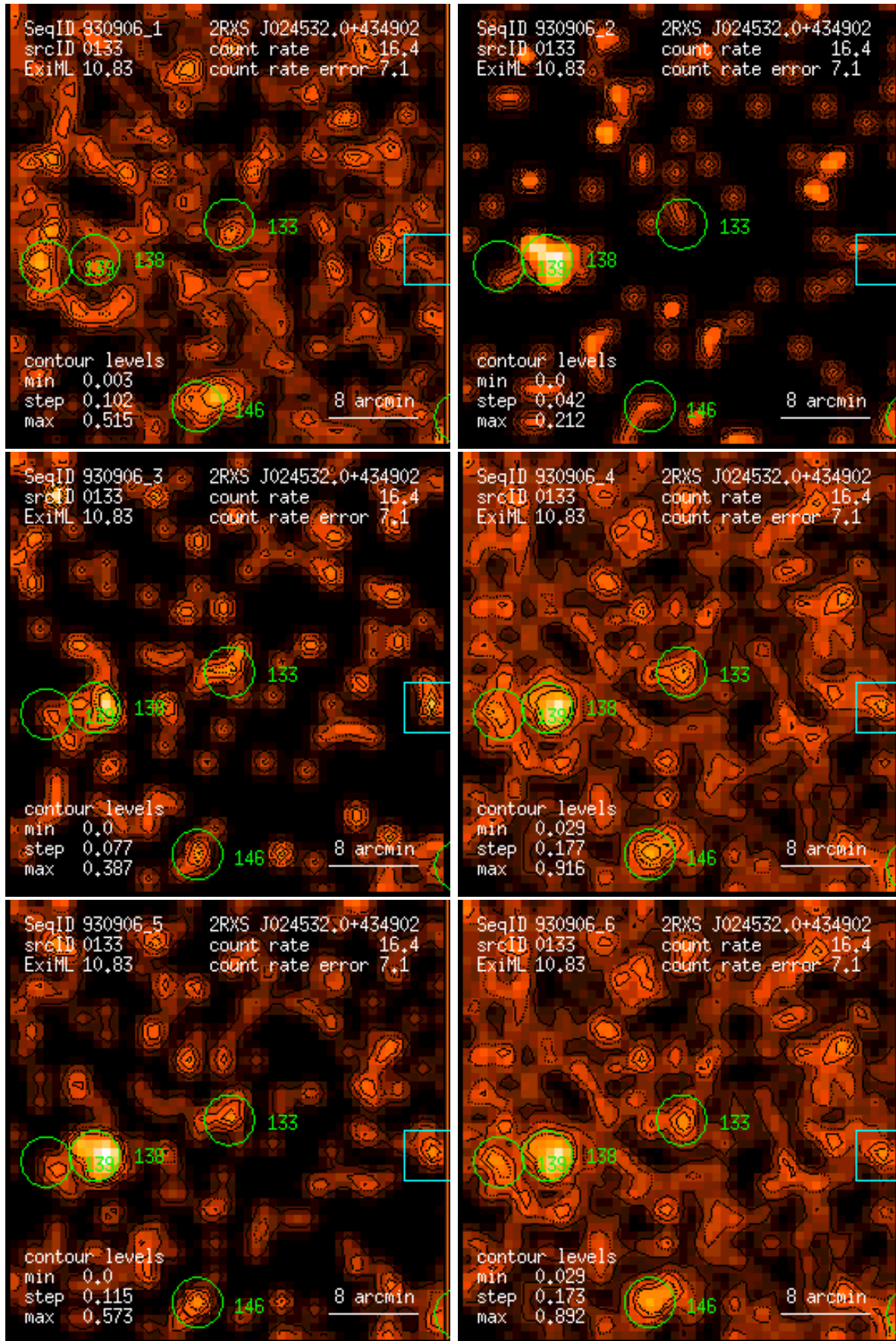
Figure 133: RASS 930906: detection 0133: band rate images, Gaussian filter: (1) PSPC channels 11 – 41, (2) 52 – 90, (3) 91 – 201, (4) 11 – 235, (5) 52 – 201, (6) 11 – 201. Broad band rates in counts/ks. Band rate contour levels in counts/ks/arcmin 2 .
