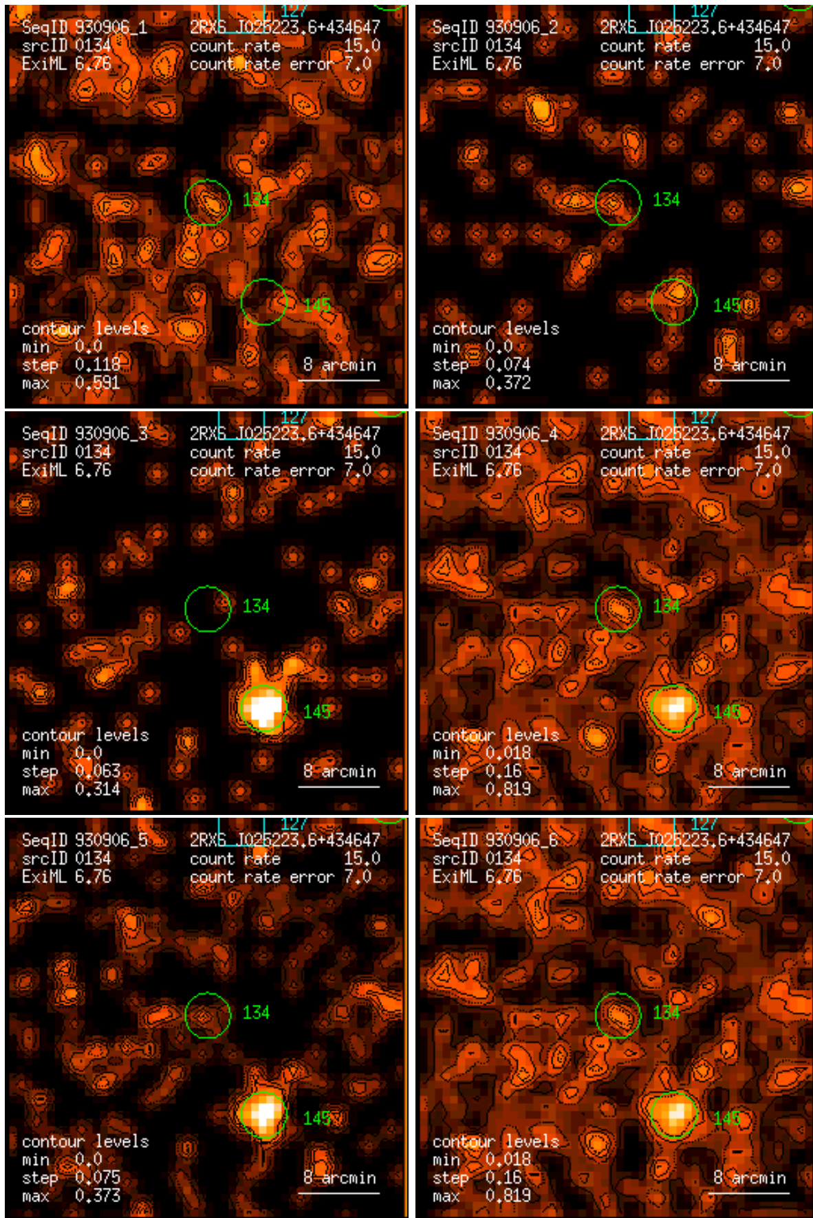
Figure 134: RASS 930906: detection 0134: band rate images, Gaussian filter: (1) PSPC channels 11 – 41, (2) 52 – 90, (3) 91 – 201, (4) 11 – 235, (5) 52 – 201, (6) 11 – 201. Broad band rates in counts/ks. Band rate contour levels in counts/ks/arcmin 2 .
