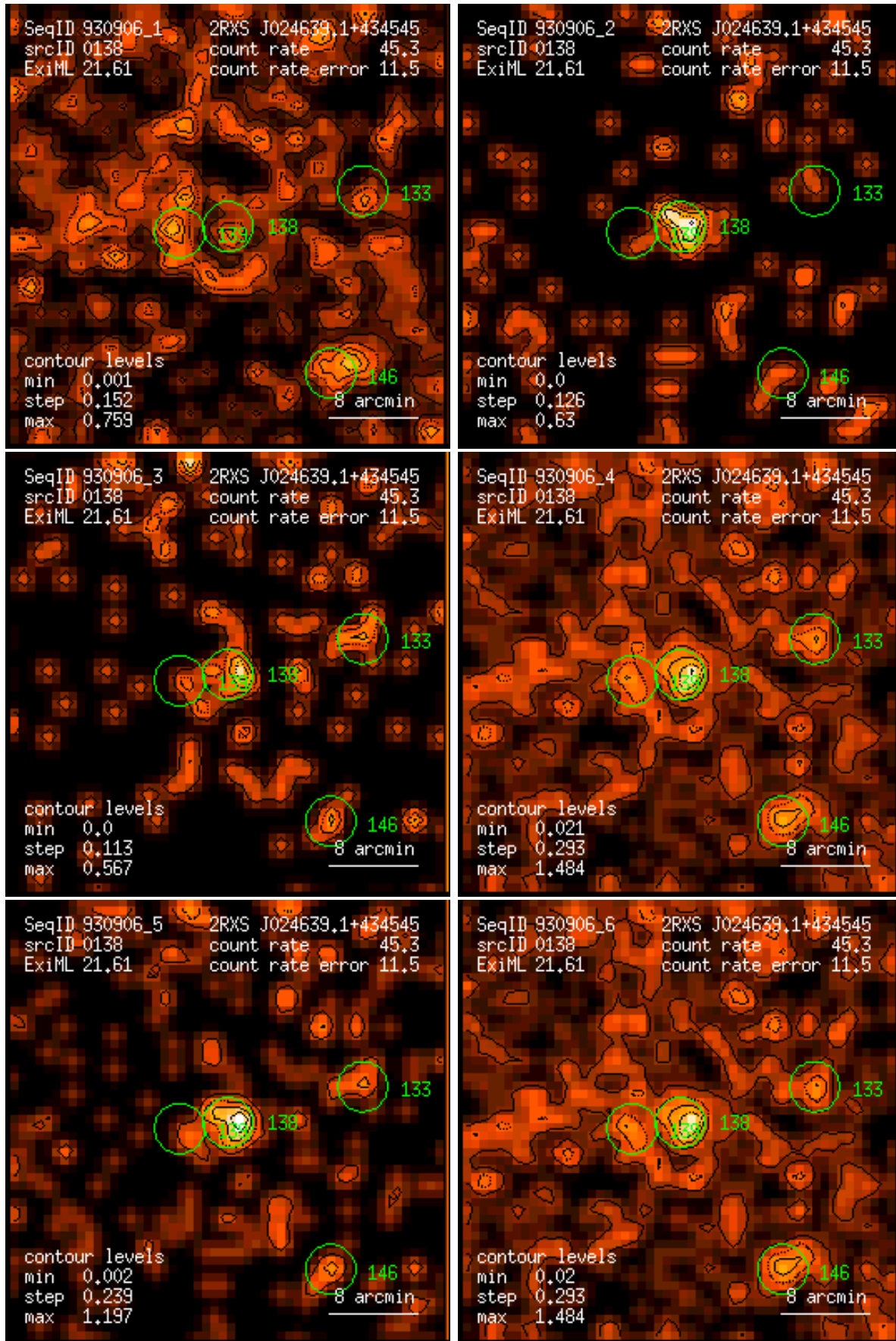
Figure 138: RASS 930906: detection 0138: band rate images, Gaussian filter: (1) PSPC channels 11 – 41, (2) 52 – 90, (3) 91 – 201, (4) 11 – 235, (5) 52 – 201, (6) 11 – 201. Broad band rates in counts/ks. Band rate contour levels in counts/ks/arcmin 2 .
