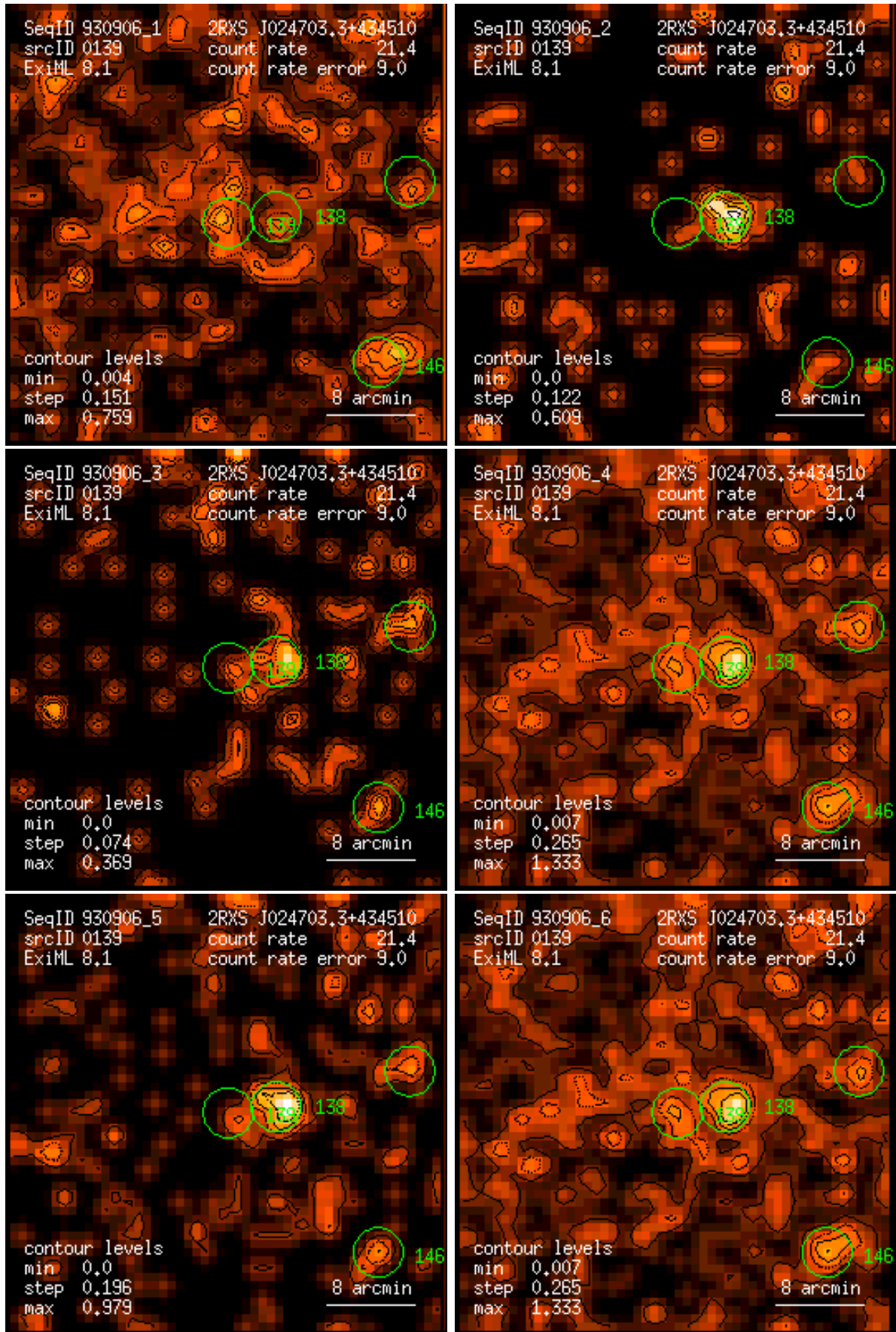
Figure 139: RASS 930906: detection 0139: band rate images, Gaussian filter: (1) PSPC channels 11 – 41, (2) 52 – 90, (3) 91 – 201, (4) 11 – 235, (5) 52 – 201, (6) 11 – 201. Broad band rates in counts/ks. Band rate contour levels in counts/ks/arcmin 2 .
