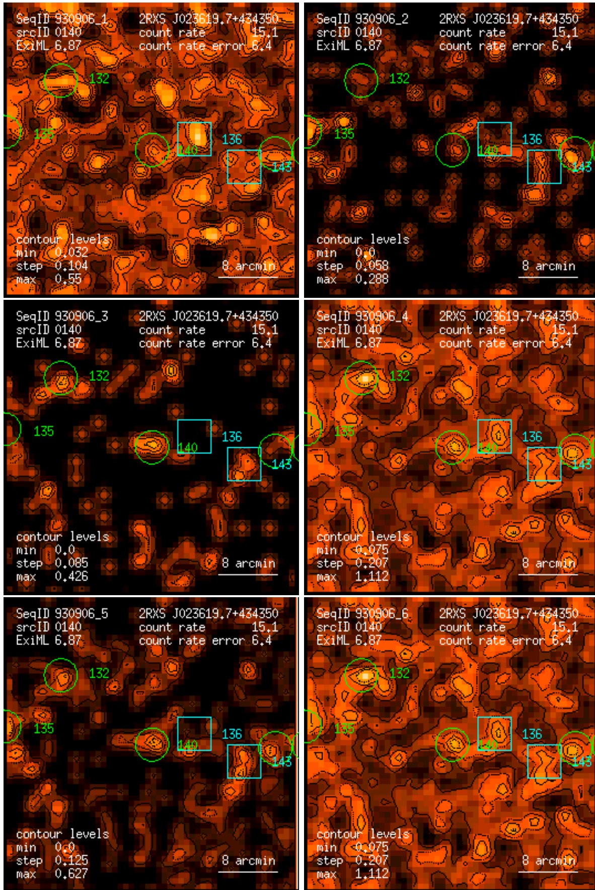
Figure 140: RASS 930906: detection 0140: band rate images, Gaussian filter: (1) PSPC channels 11 – 41, (2) 52 – 90, (3) 91 – 201, (4) 11 – 235, (5) 52 – 201, (6) 11 – 201. Broad band rates in counts/ks. Band rate contour levels in counts/ks/arcmin 2 .
