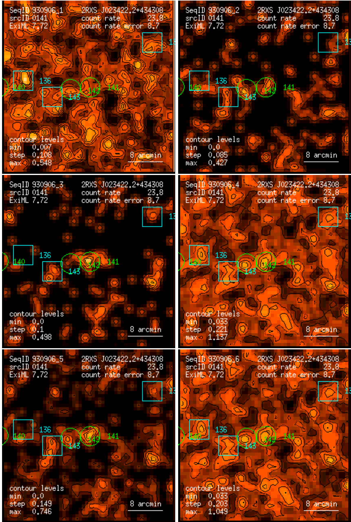
Figure 141: RASS 930906: detection 0141: band rate images, Gaussian filter: (1) PSPC channels 11 – 41, (2) 52 – 90, (3) 91 – 201, (4) 11 – 235, (5) 52 – 201, (6) 11 – 201. Broad band rates in counts/ks. Band rate contour levels in counts/ks/arcmin 2 .
