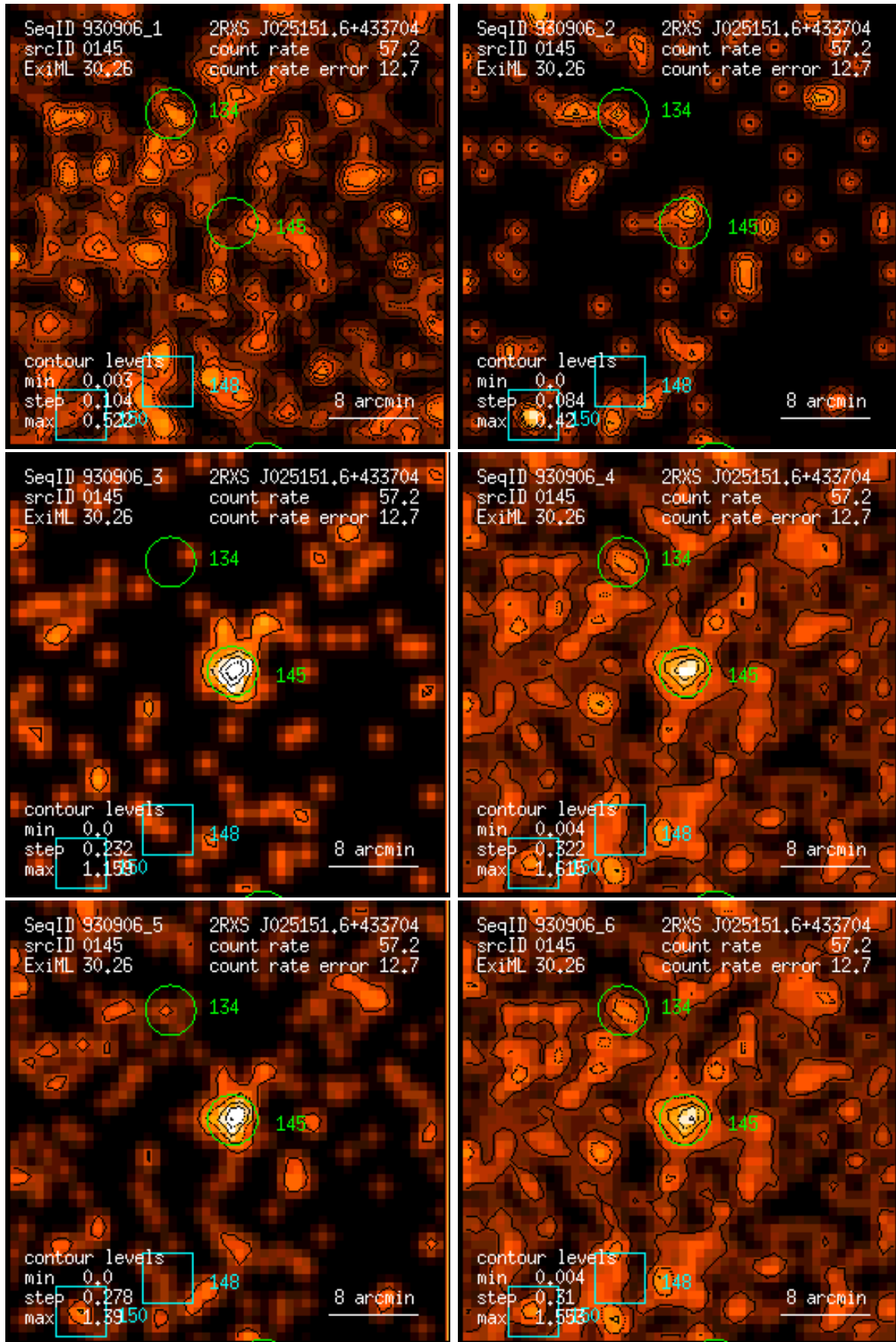
Figure 145: RASS 930906: detection 0145: band rate images, Gaussian filter: (1) PSPC channels 11 – 41, (2) 52 – 90, (3) 91 – 201, (4) 11 – 235, (5) 52 – 201, (6) 11 – 201. Broad band rates in counts/ks. Band rate contour levels in counts/ks/arcmin 2 .
