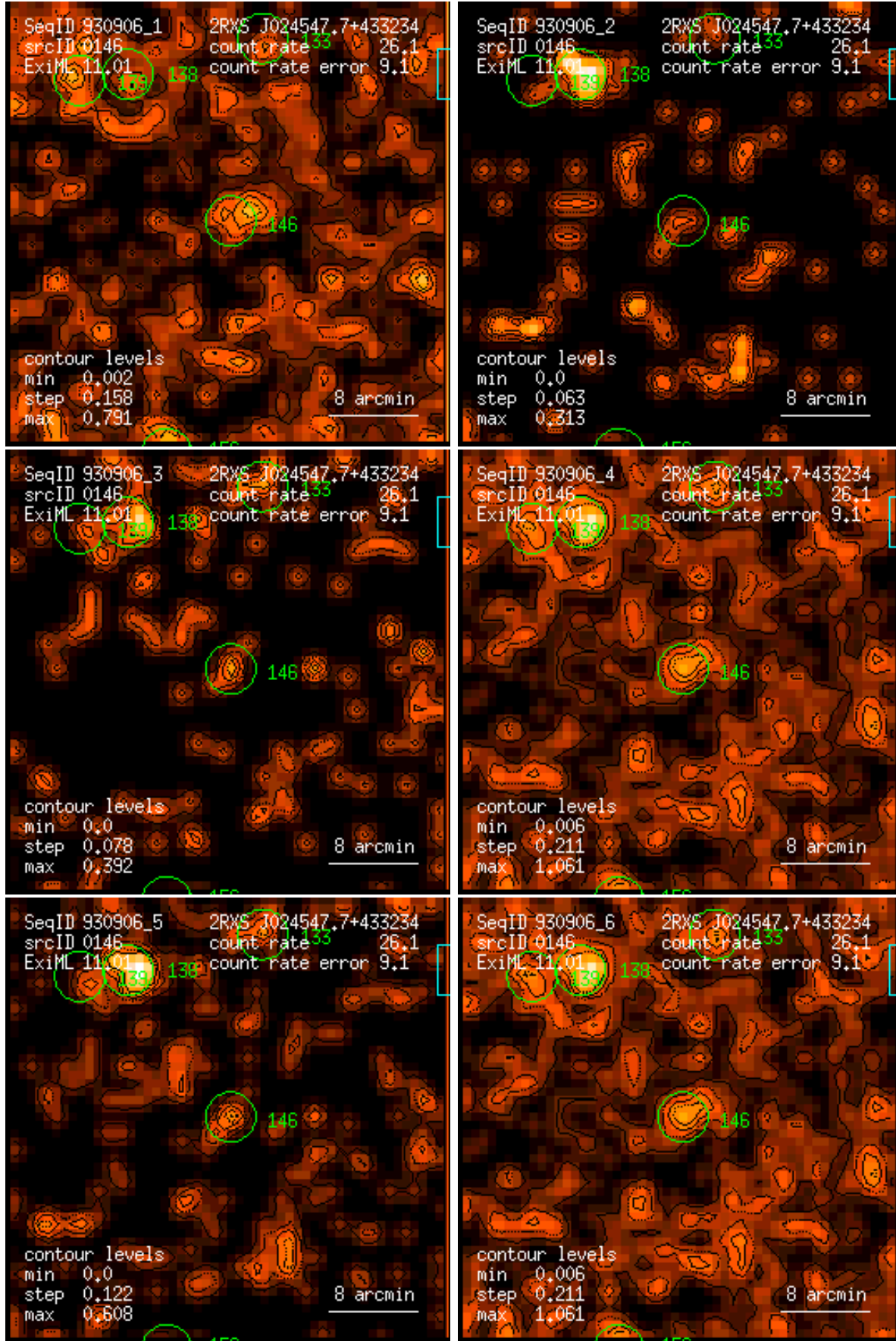
Figure 146: RASS 930906: detection 0146: band rate images, Gaussian filter: (1) PSPC channels 11 – 41, (2) 52 – 90, (3) 91 – 201, (4) 11 – 235, (5) 52 – 201, (6) 11 – 201. Broad band rates in counts/ks. Band rate contour levels in counts/ks/arcmin 2 .
