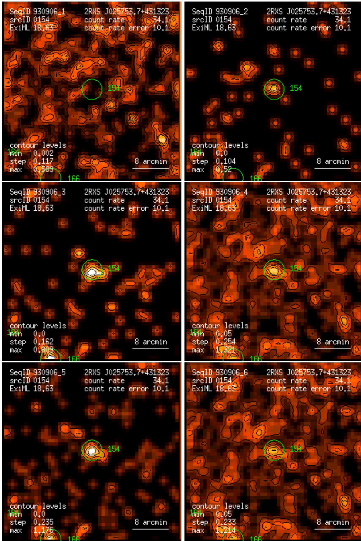
Figure 154: RASS 930906: detection 0154: band rate images, Gaussian filter: (1) PSPC channels 11 – 41, (2) 52 – 90, (3) 91 – 201, (4) 11 – 235, (5) 52 – 201, (6) 11 – 201. Broad band rates in counts/ks. Band rate contour levels in counts/ks/arcmin 2 .
