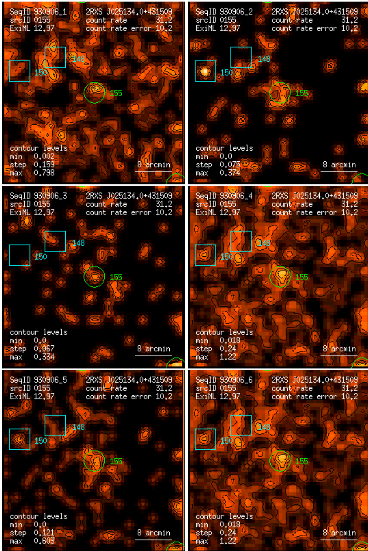
Figure 155: RASS 930906: detection 0155: band rate images, Gaussian filter: (1) PSPC channels 11 – 41, (2) 52 – 90, (3) 91 – 201, (4) 11 – 235, (5) 52 – 201, (6) 11 – 201. Broad band rates in counts/ks. Band rate contour levels in counts/ks/arcmin 2 .
