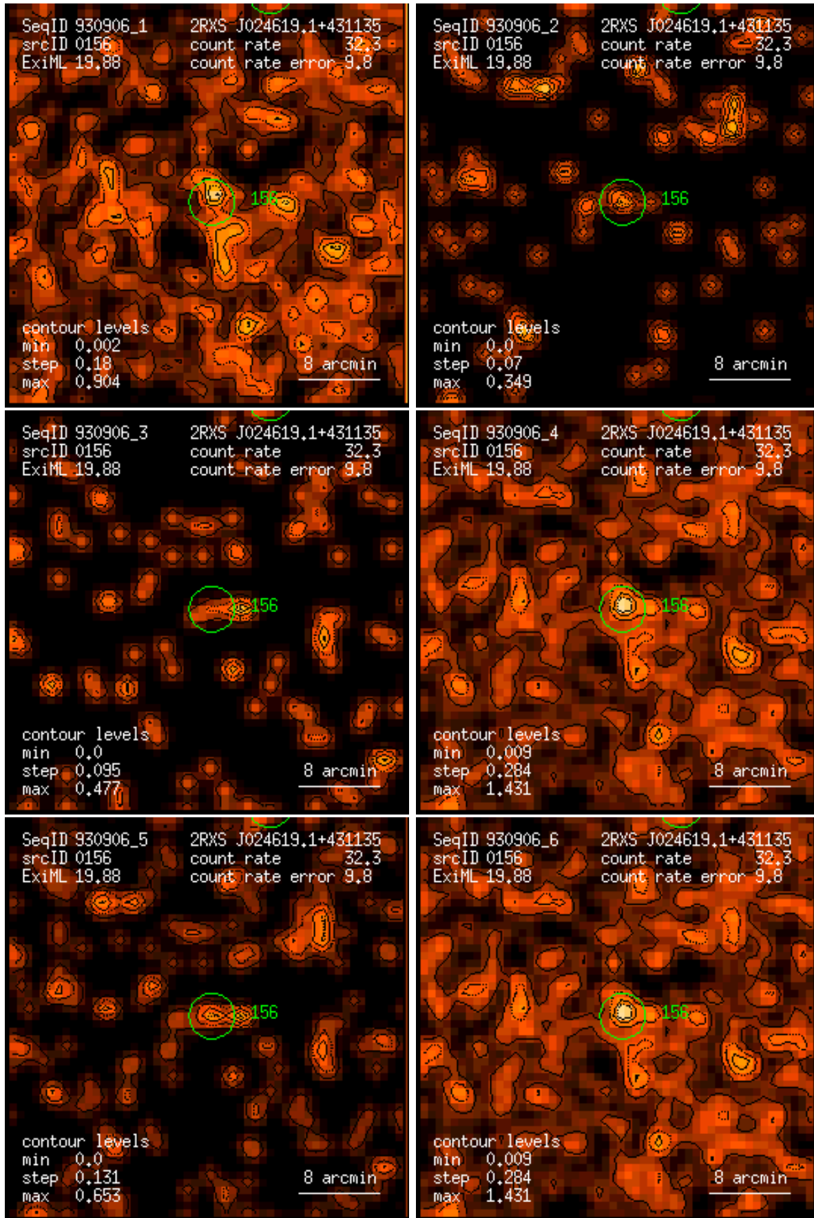
Figure 156: RASS 930906: detection 0156: band rate images, Gaussian filter: (1) PSPC channels 11 – 41, (2) 52 – 90, (3) 91 – 201, (4) 11 – 235, (5) 52 – 201, (6) 11 – 201. Broad band rates in counts/ks. Band rate contour levels in counts/ks/arcmin 2 .
