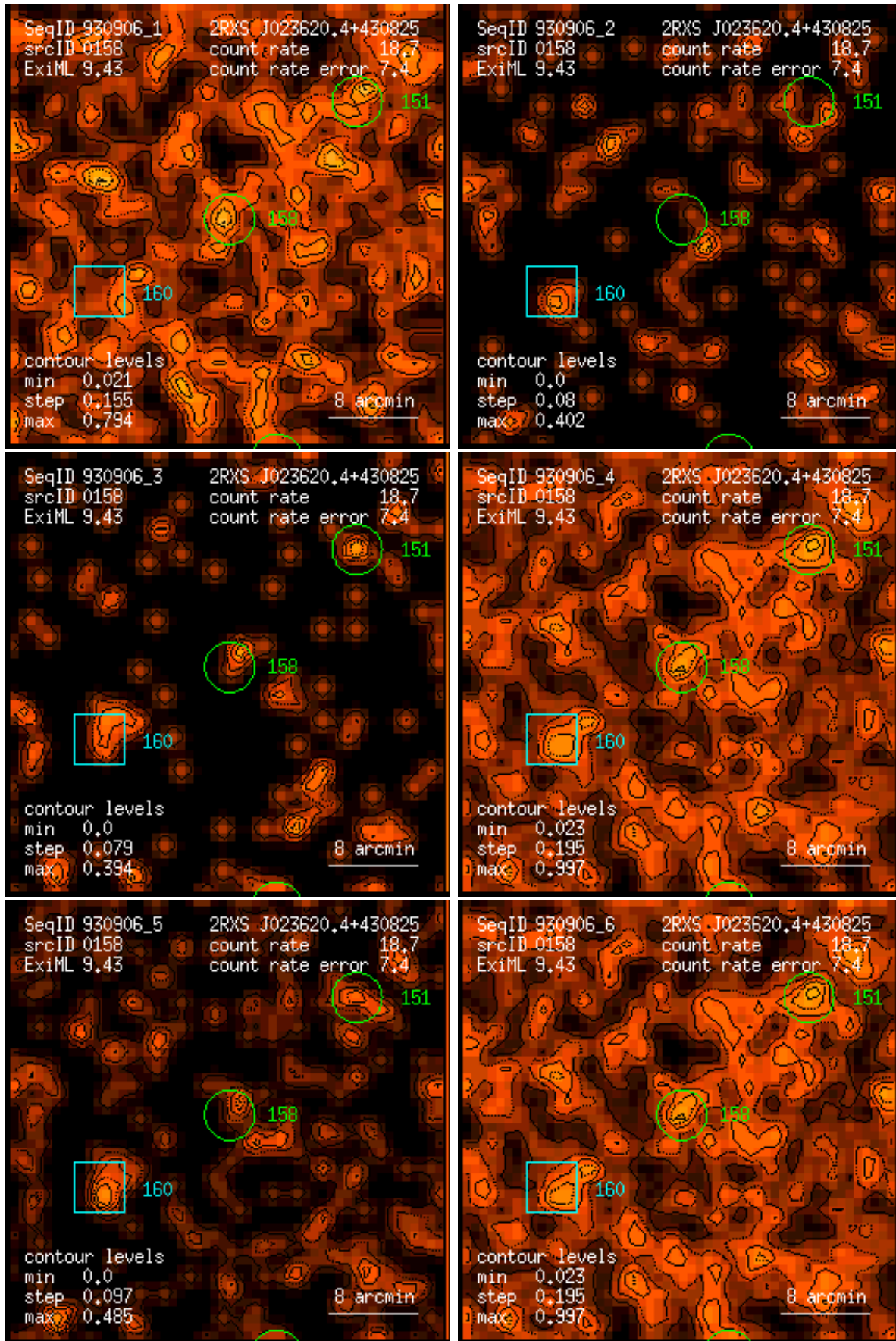
Figure 158: RASS 930906: detection 0158: band rate images, Gaussian filter: (1) PSPC channels 11 – 41, (2) 52 – 90, (3) 91 – 201, (4) 11 – 235, (5) 52 – 201, (6) 11 – 201. Broad band rates in counts/ks. Band rate contour levels in counts/ks/arcmin 2 .
