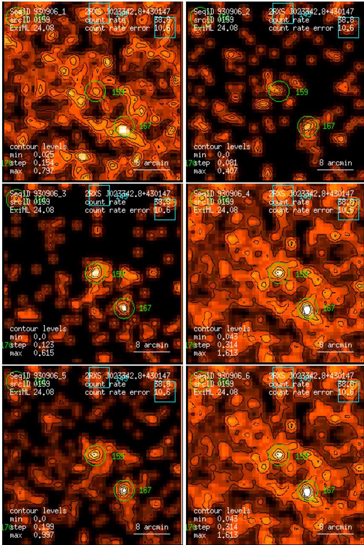
Figure 159: RASS 930906: detection 0159: band rate images, Gaussian filter: (1) PSPC channels 11 – 41, (2) 52 – 90, (3) 91 – 201, (4) 11 – 235, (5) 52 – 201, (6) 11 – 201. Broad band rates in counts/ks. Band rate contour levels in counts/ks/arcmin 2 .
