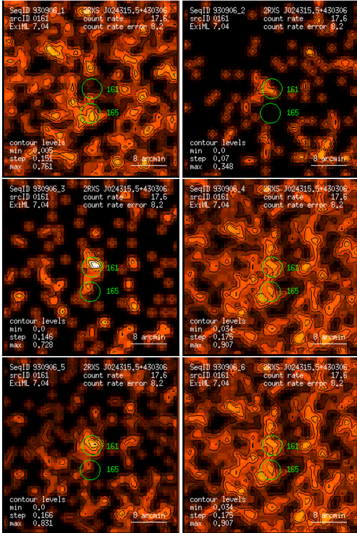
Figure 161: RASS 930906: detection 0161: band rate images, Gaussian filter: (1) PSPC channels 11 – 41, (2) 52 – 90, (3) 91 – 201, (4) 11 – 235, (5) 52 – 201, (6) 11 – 201. Broad band rates in counts/ks. Band rate contour levels in counts/ks/arcmin 2 .
