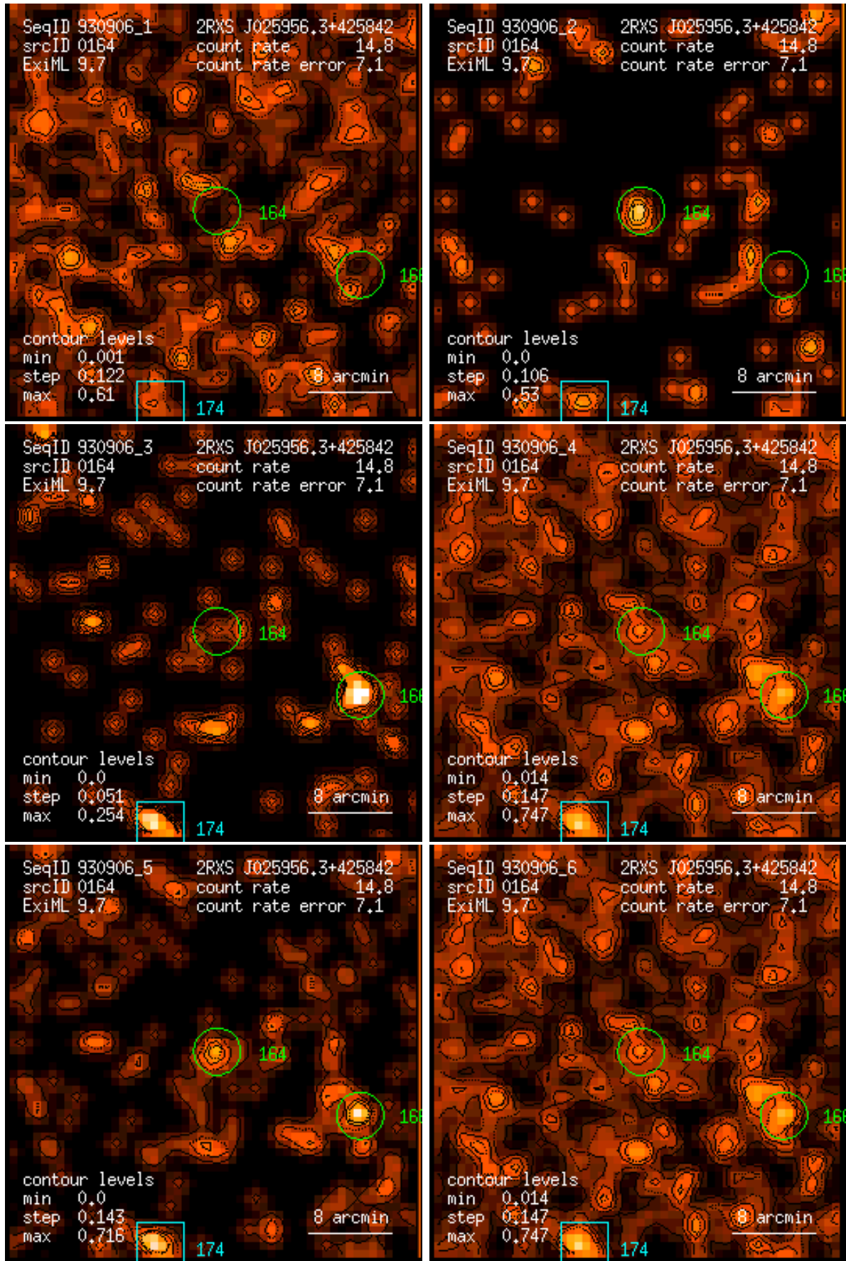
Figure 164: RASS 930906: detection 0164: band rate images, Gaussian filter: (1) PSPC channels 11 – 41, (2) 52 – 90, (3) 91 – 201, (4) 11 – 235, (5) 52 – 201, (6) 11 – 201. Broad band rates in counts/ks. Band rate contour levels in counts/ks/arcmin 2 .
