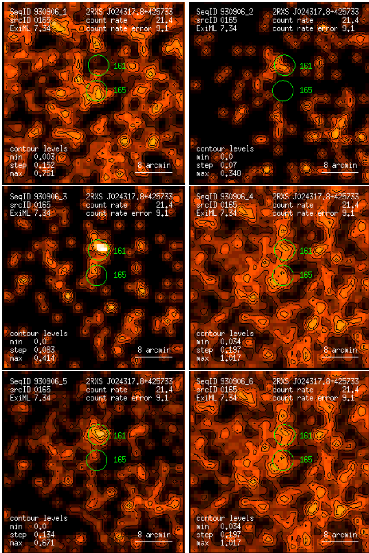
Figure 165: RASS 930906: detection 0165: band rate images, Gaussian filter: (1) PSPC channels 11 – 41, (2) 52 – 90, (3) 91 – 201, (4) 11 – 235, (5) 52 – 201, (6) 11 – 201. Broad band rates in counts/ks. Band rate contour levels in counts/ks/arcmin 2 .
