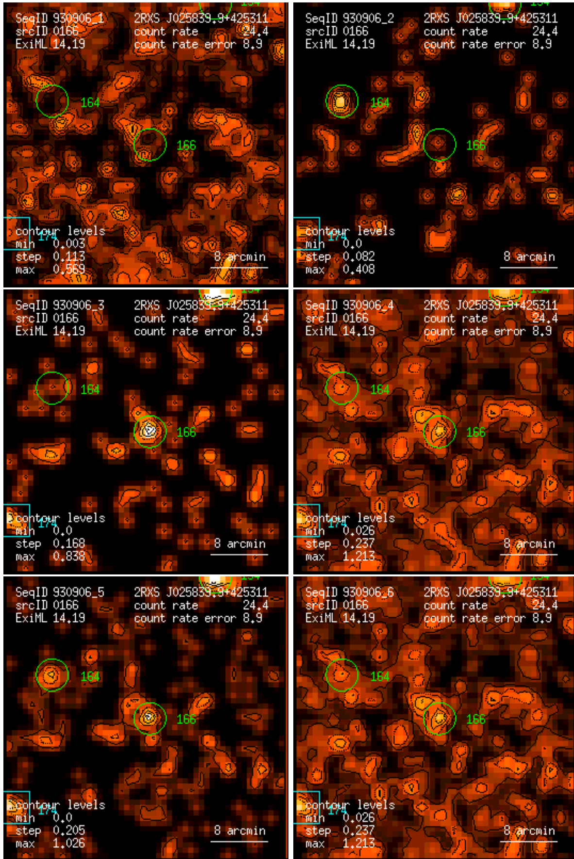
Figure 166: RASS 930906: detection 0166: band rate images, Gaussian filter: (1) PSPC channels 11 – 41, (2) 52 – 90, (3) 91 – 201, (4) 11 – 235, (5) 52 – 201, (6) 11 – 201. Broad band rates in counts/ks. Band rate contour levels in counts/ks/arcmin 2 .
