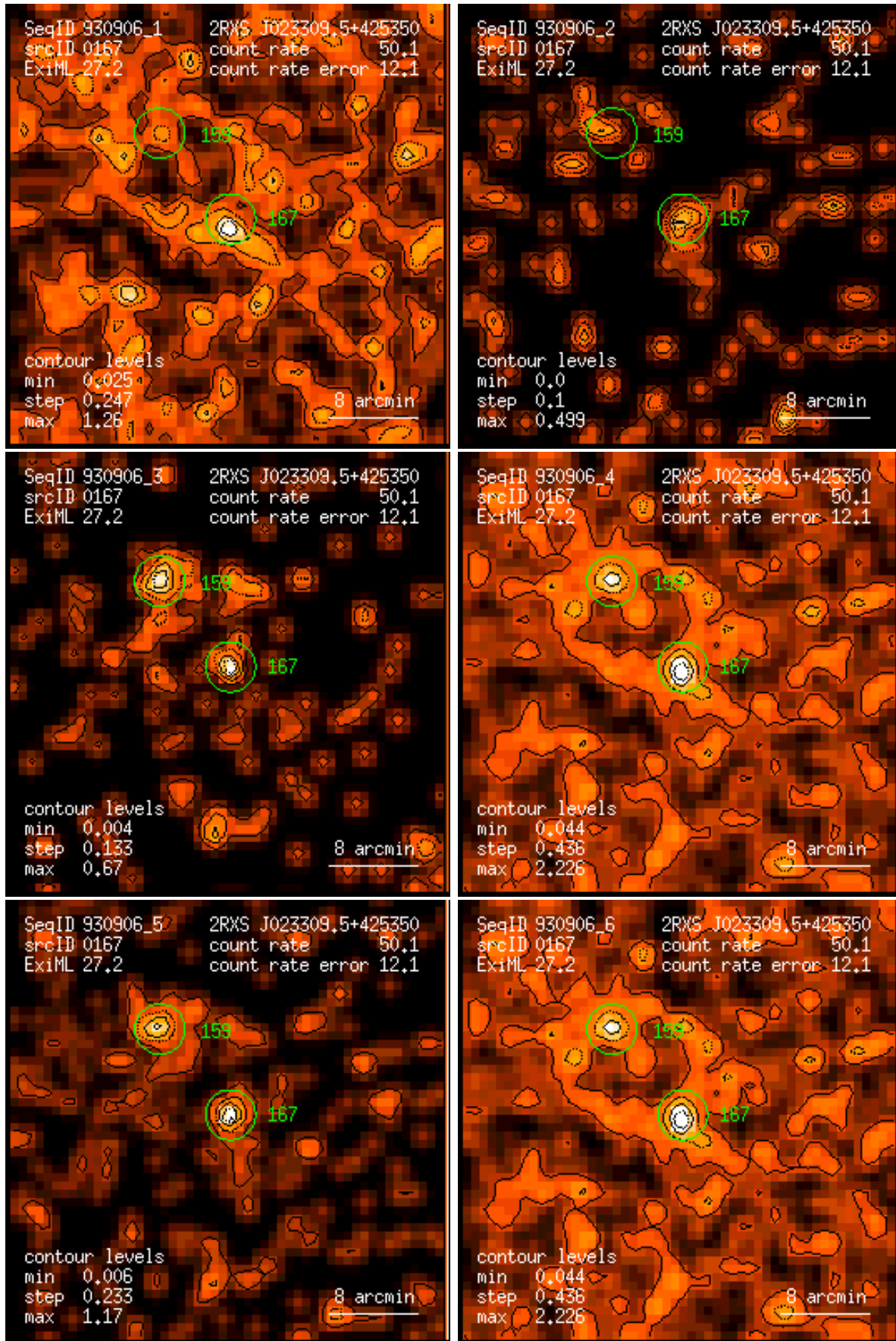
Figure 167: RASS 930906: detection 0167: band rate images, Gaussian filter: (1) PSPC channels 11 – 41, (2) 52 – 90, (3) 91 – 201, (4) 11 – 235, (5) 52 – 201, (6) 11 – 201. Broad band rates in counts/ks. Band rate contour levels in counts/ks/arcmin 2 .
