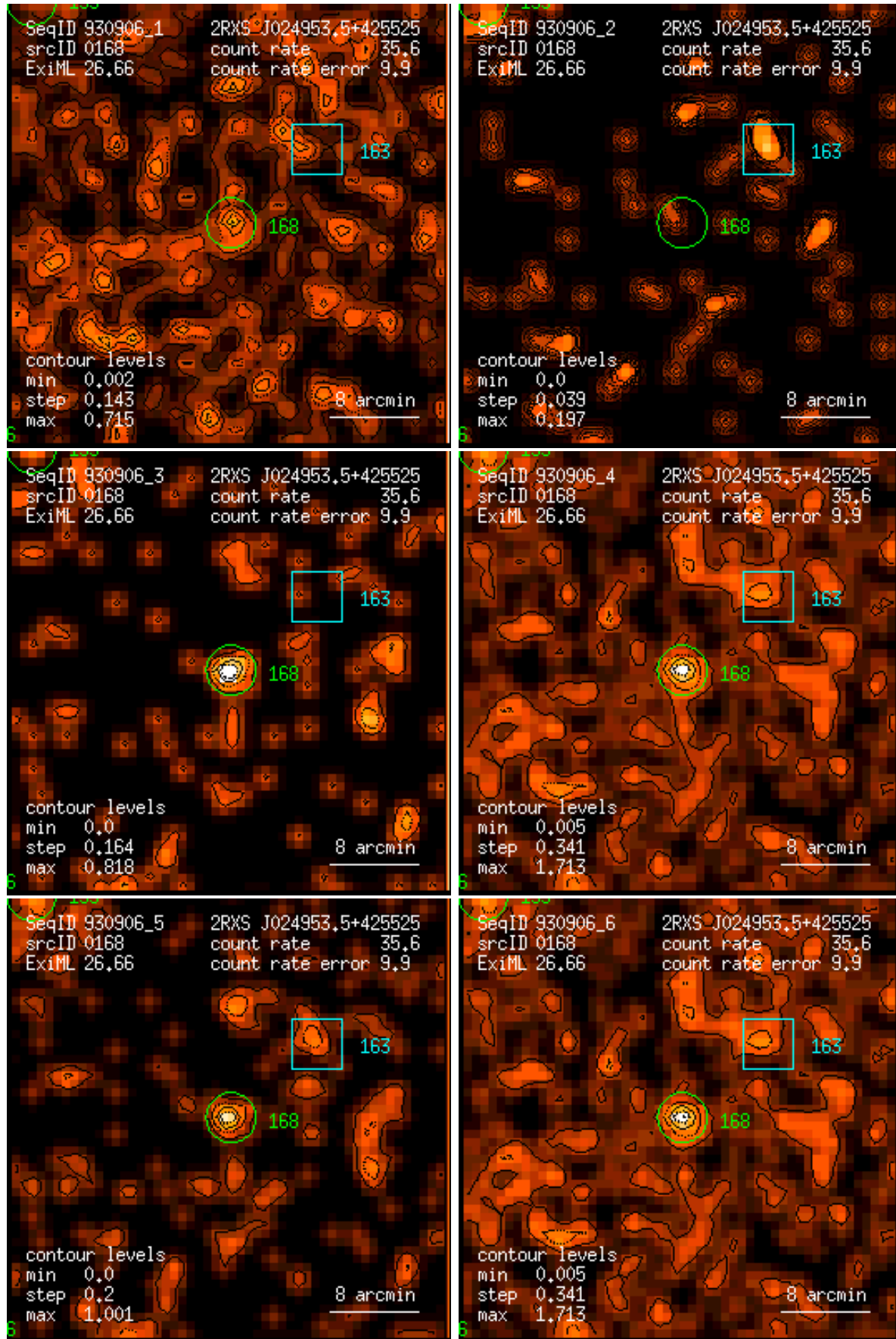
Figure 168: RASS 930906: detection 0168: band rate images, Gaussian filter: (1) PSPC channels 11 – 41, (2) 52 – 90, (3) 91 – 201, (4) 11 – 235, (5) 52 – 201, (6) 11 – 201. Broad band rates in counts/ks. Band rate contour levels in counts/ks/arcmin 2 .
