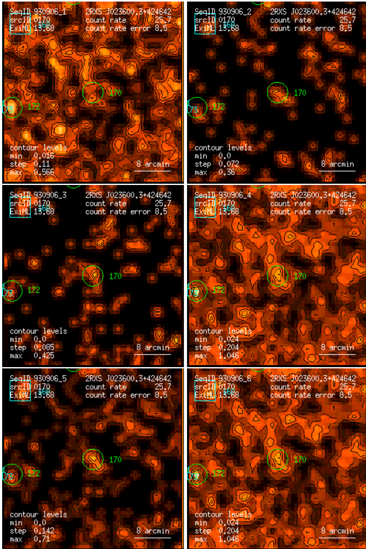
Figure 170: RASS 930906: detection 0170: band rate images, Gaussian filter: (1) PSPC channels 11 – 41, (2) 52 – 90, (3) 91 – 201, (4) 11 – 235, (5) 52 – 201, (6) 11 – 201. Broad band rates in counts/ks. Band rate contour levels in counts/ks/arcmin 2 .
