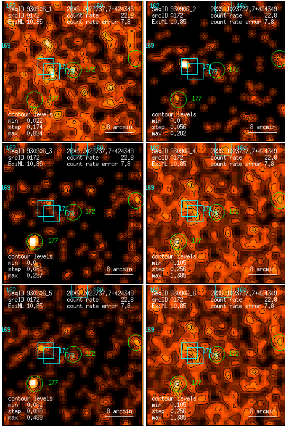
Figure 172: RASS 930906: detection 0172: band rate images, Gaussian filter: (1) PSPC channels 11 – 41, (2) 52 – 90, (3) 91 – 201, (4) 11 – 235, (5) 52 – 201, (6) 11 – 201. Broad band rates in counts/ks. Band rate contour levels in counts/ks/arcmin 2 .
