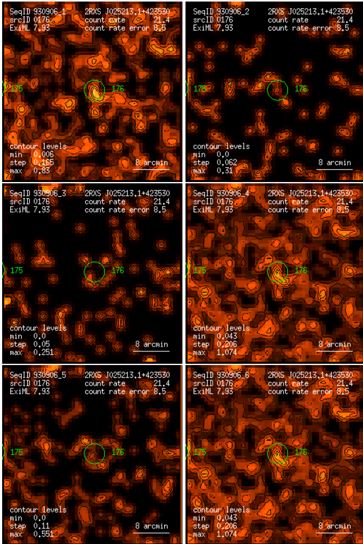
Figure 176: RASS 930906: detection 0176: band rate images, Gaussian filter: (1) PSPC channels 11 – 41, (2) 52 – 90, (3) 91 – 201, (4) 11 – 235, (5) 52 – 201, (6) 11 – 201. Broad band rates in counts/ks. Band rate contour levels in counts/ks/arcmin 2 .
