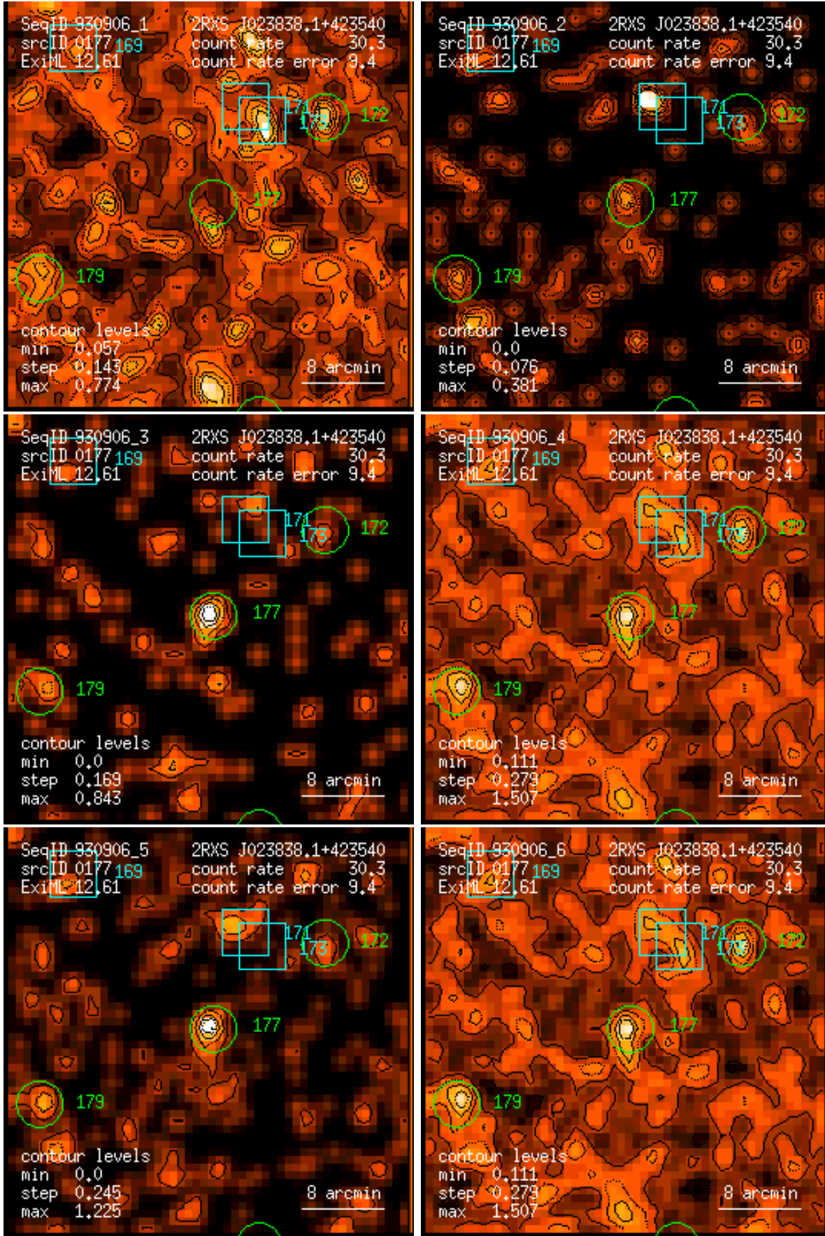
Figure 177: RASS 930906: detection 0177: band rate images, Gaussian filter: (1) PSPC channels 11 – 41, (2) 52 – 90, (3) 91 – 201, (4) 11 – 235, (5) 52 – 201, (6) 11 – 201. Broad band rates in counts/ks. Band rate contour levels in counts/ks/arcmin 2 .
