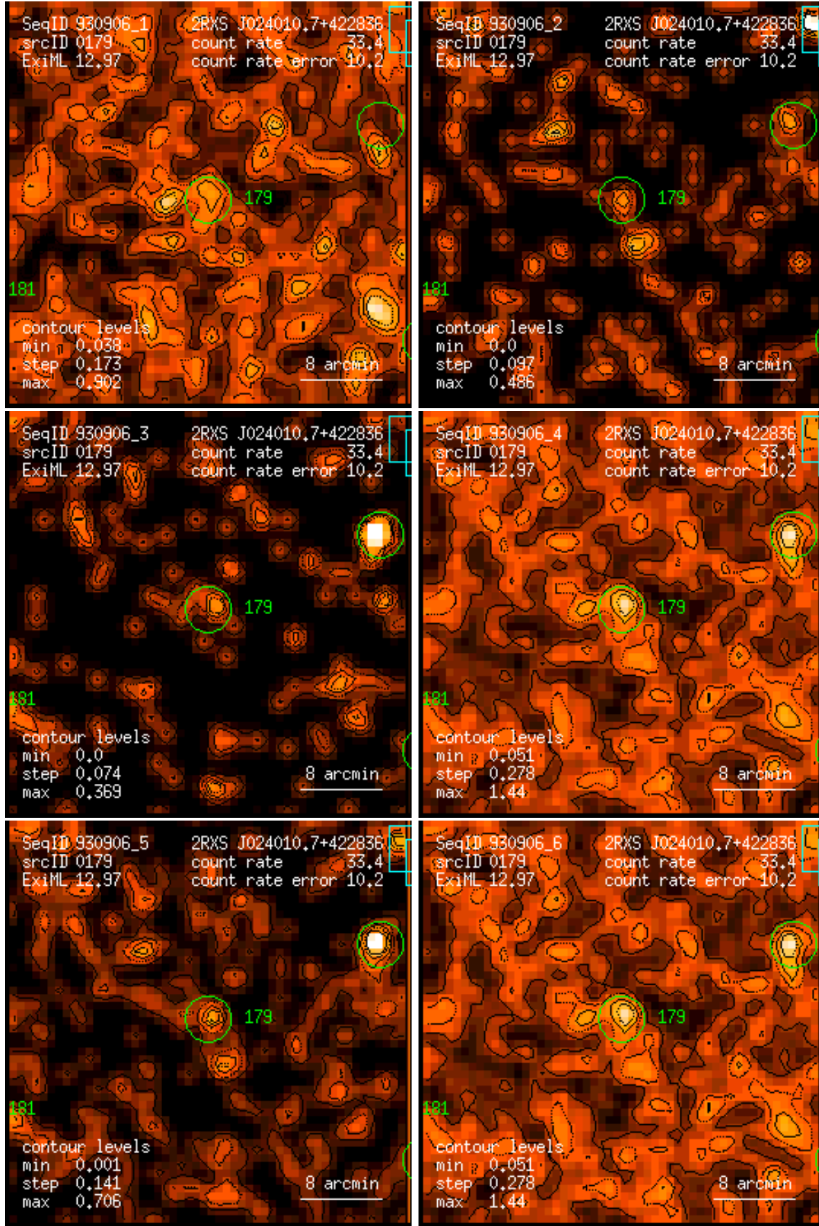
Figure 179: RASS 930906: detection 0179: band rate images, Gaussian filter: (1) PSPC channels 11 – 41, (2) 52 – 90, (3) 91 – 201, (4) 11 – 235, (5) 52 – 201, (6) 11 – 201. Broad band rates in counts/ks. Band rate contour levels in counts/ks/arcmin 2 .
