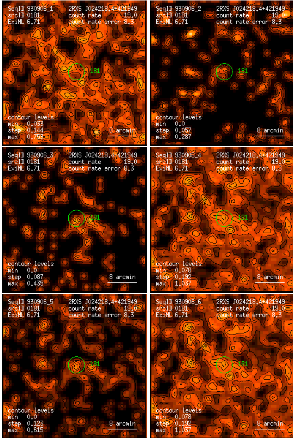
Figure 181: RASS 930906: detection 0181: band rate images, Gaussian filter: (1) PSPC channels 11 – 41, (2) 52 – 90, (3) 91 – 201, (4) 11 – 235, (5) 52 – 201, (6) 11 – 201. Broad band rates in counts/ks. Band rate contour levels in counts/ks/arcmin 2 .
