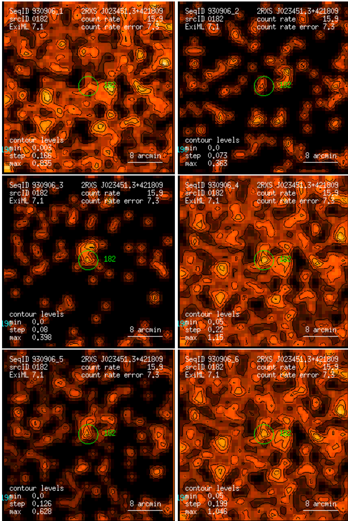
Figure 182: RASS 930906: detection 0182: band rate images, Gaussian filter: (1) PSPC channels 11 – 41, (2) 52 – 90, (3) 91 – 201, (4) 11 – 235, (5) 52 – 201, (6) 11 – 201. Broad band rates in counts/ks. Band rate contour levels in counts/ks/arcmin 2 .
