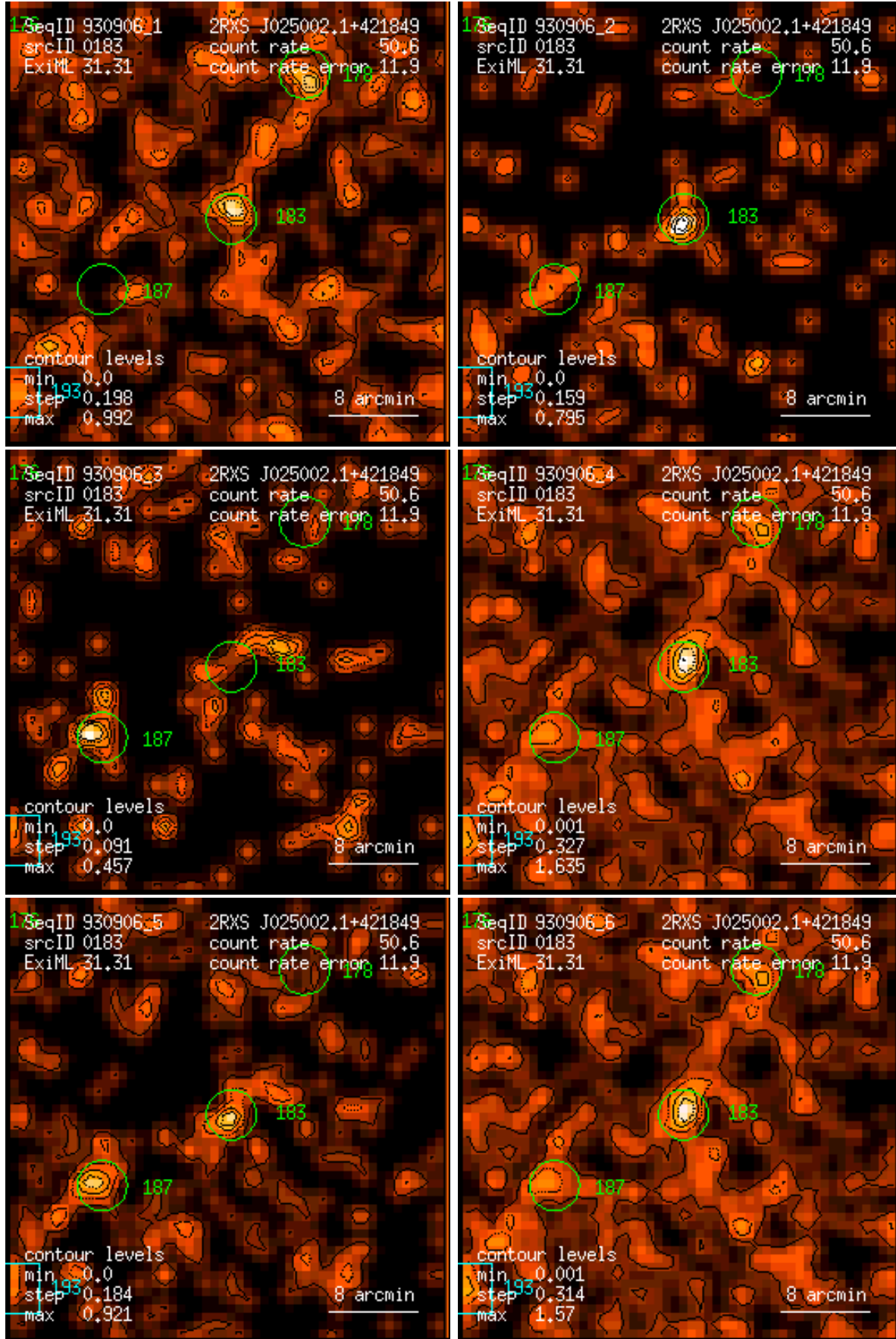
Figure 183: RASS 930906: detection 0183: band rate images, Gaussian filter: (1) PSPC channels 11 – 41, (2) 52 – 90, (3) 91 – 201, (4) 11 – 235, (5) 52 – 201, (6) 11 – 201. Broad band rates in counts/ks. Band rate contour levels in counts/ks/arcmin 2 .
